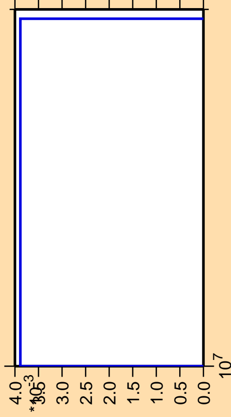
\Delta\sigma/\sigma vs. E for ^{98}\text{Ru}(n,pt)
