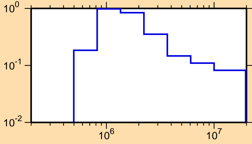
\sigma vs. E for ^{98}\text{Ru}(n,n_1)
