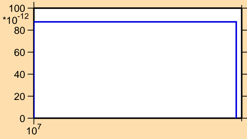
\sigma vs. E for ^{98}\text{Ru}(n,pd)
