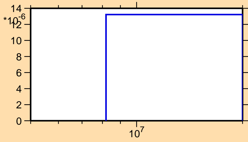
\sigma vs. E for ^{98}\text{Ru}(n,t)
