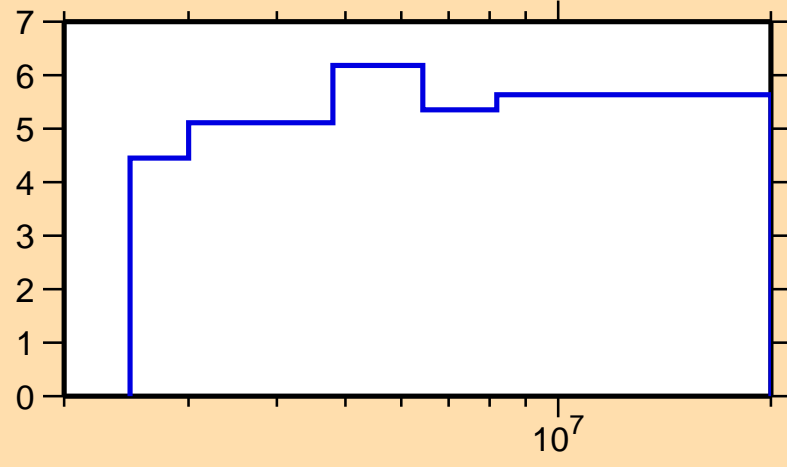
\Delta\sigma/\sigma vs. E for ^{98}\text{Ru}(n, n\text{nonel.})
