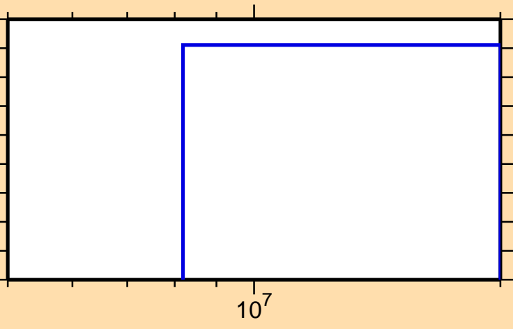
\sigma vs. E for ^{98}\text{Ru}(n,\text{He}3)
