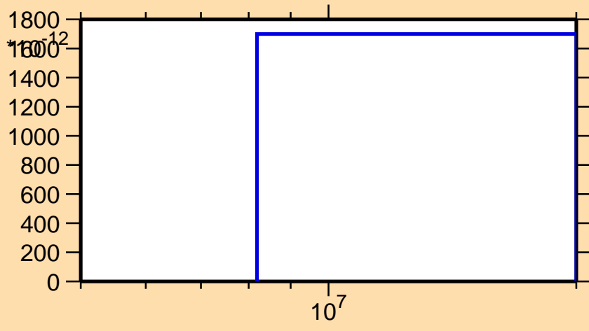
\sigma vs. E for ^{98}\text{Ru}(n,\text{nd})
