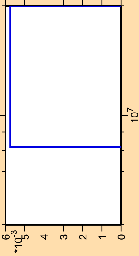
\Delta\sigma/\sigma vs. E for ^{98}\text{Ru}(n,\text{pt})
