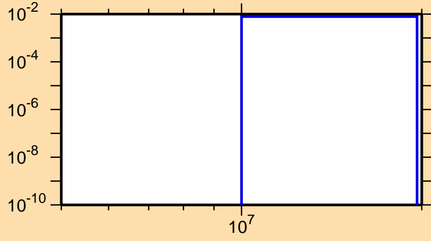
\sigma vs. E for ^{100}\text{Ru}(n,np)
