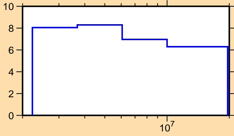
\Delta\sigma/\sigma vs. E for ^{100}\text{Ru}(n,n\text{onel.})
