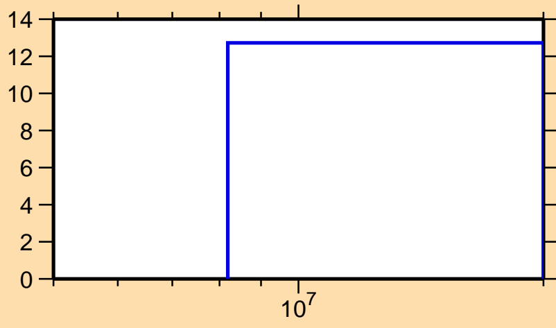
\Delta\sigma/\sigma vs. E for ^{100}\text{Ru}(n,2n)
