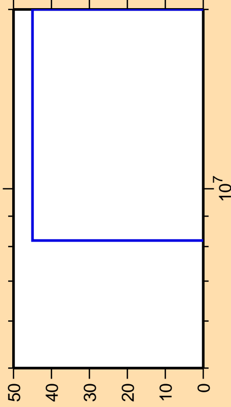
\Delta\sigma/\sigma vs. E for ^{100}\text{Ru}(n,p)
