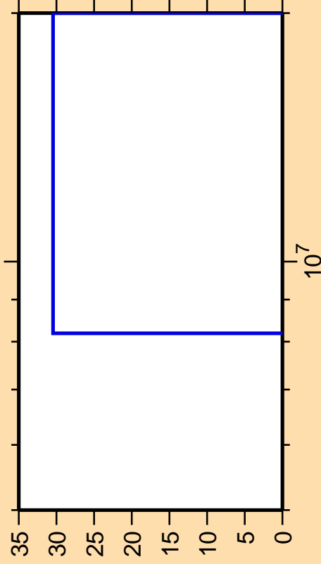
\Delta\sigma/\sigma vs. E for ^{100}\text{Ru}(n,n_1)
