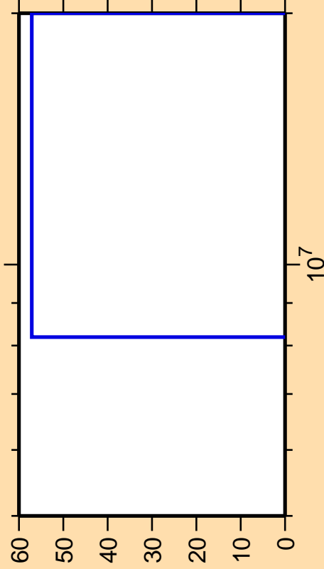
\Delta\sigma/\sigma vs. E for ^{100}\text{Ru}(n,\alpha)
