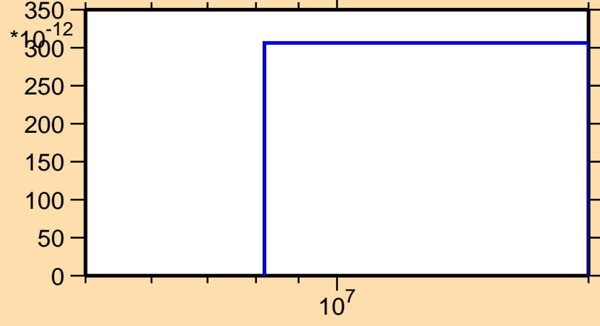
\sigma vs. E for ^{100}\text{Ru}(n,nd)
