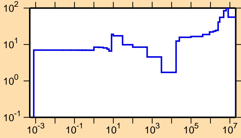
\Delta\sigma/\sigma vs. E for ^{100}\text{Ru}(n,\gamma)
