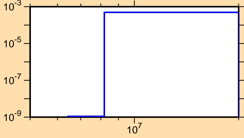
\sigma vs. E for ^{100}\text{Ru}(n,n\alpha)
