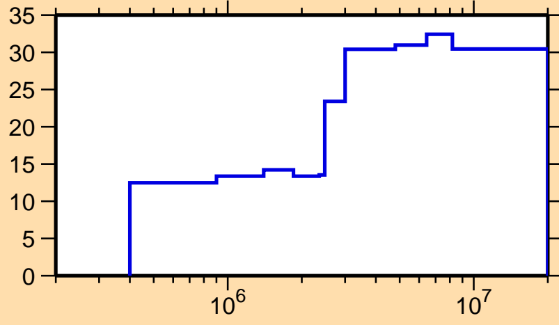
\Delta\sigma/\sigma vs. E for ^{100}\text{Ru}(n,n_1)
