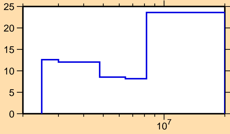
\Delta\sigma/\sigma vs. E for ^{100}\text{Ru}(n,n\text{cont.})
