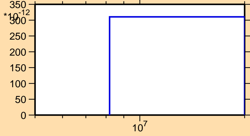
\sigma vs. E for ^{100}\text{Ru}(n,2n\alpha)
