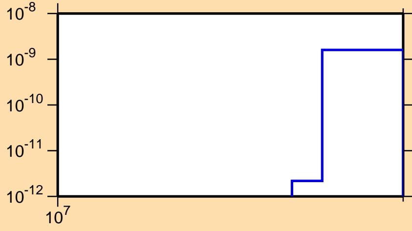
\sigma vs. E for ^{102}\text{Ru}(n,2n\alpha)
