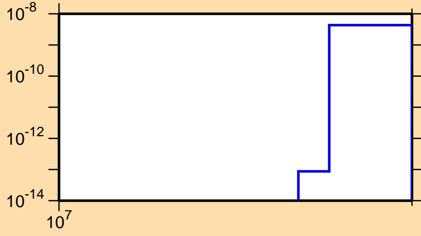
\sigma vs. E for ^{102}\text{Ru}(n,\text{nd})
