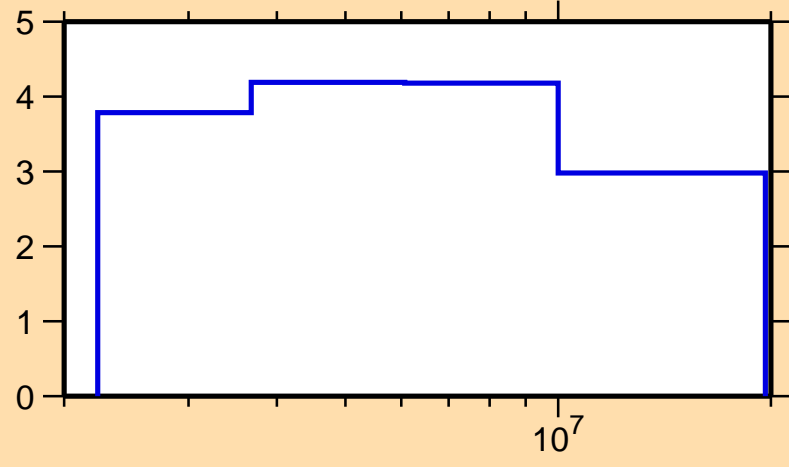
\Delta\sigma/\sigma vs. E for ^{102}\text{Ru}(n,n\text{onel.})
