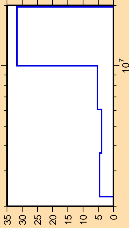
\Delta\sigma/\sigma vs. E for ^{102}\text{Ru}(n,n\text{cont.})
