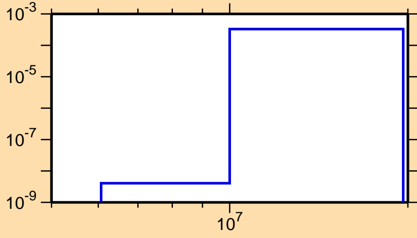
\sigma vs. E for ^{102}\text{Ru}(n,n\alpha)
