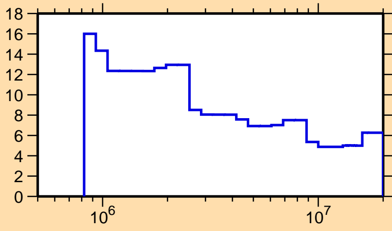
\Delta\sigma/\sigma vs. E for ^{103}\text{Ru}(n,n\text{onel.})
