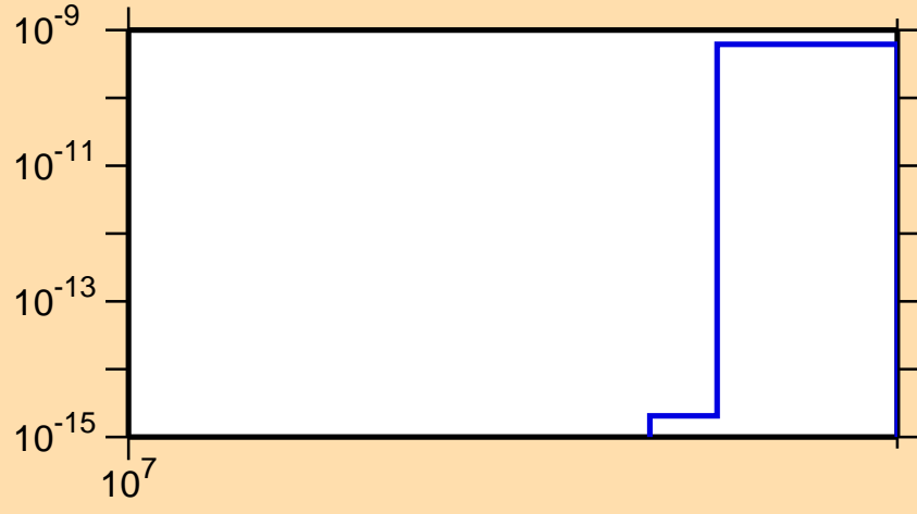
\sigma vs. E for ^{103}\text{Ru}(n,nt)
