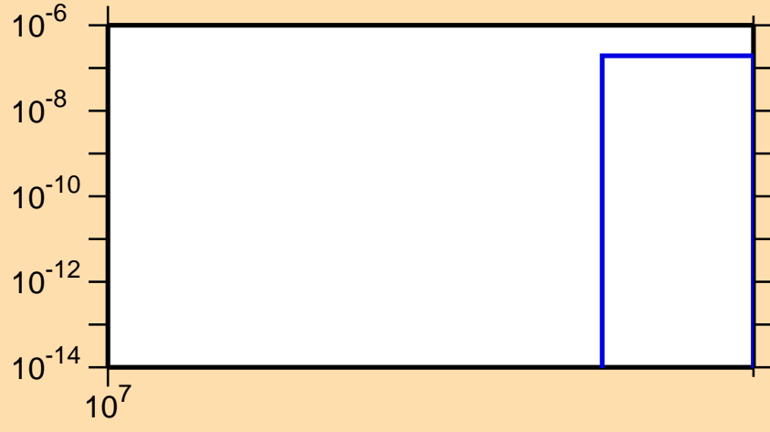
\sigma vs. E for ^{103}\text{Ru}(n,2np)
