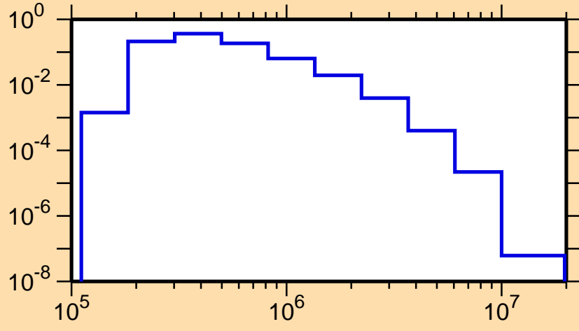
\sigma vs. E for ^{103}\text{Ru}(n,n_3)
