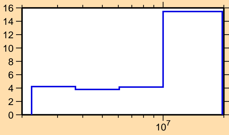
\Delta\sigma/\sigma vs. E for ^{104}\text{Ru}(n,n\text{cont.})
