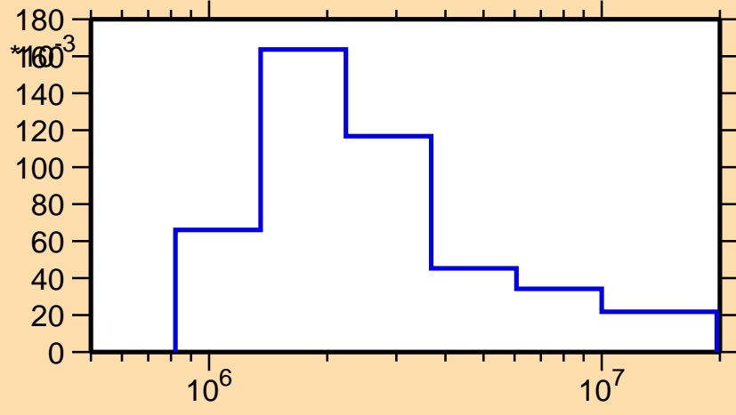
\sigma vs. E for ^{104}\text{Ru}(n,n_2)
