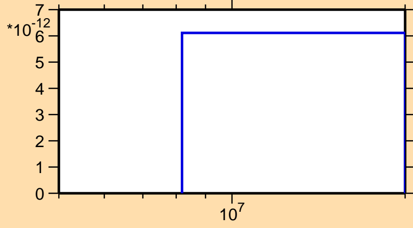
\sigma vs. E for ^{104}\text{Ru}(n,nd)
