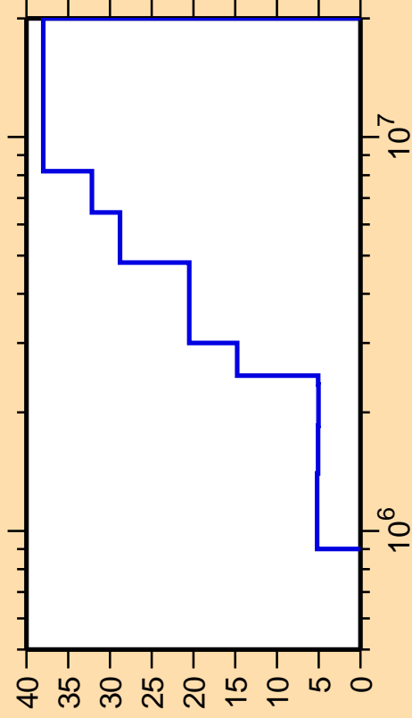
\Delta\sigma/\sigma vs. E for ^{104}\text{Ru}(n,n_3)
