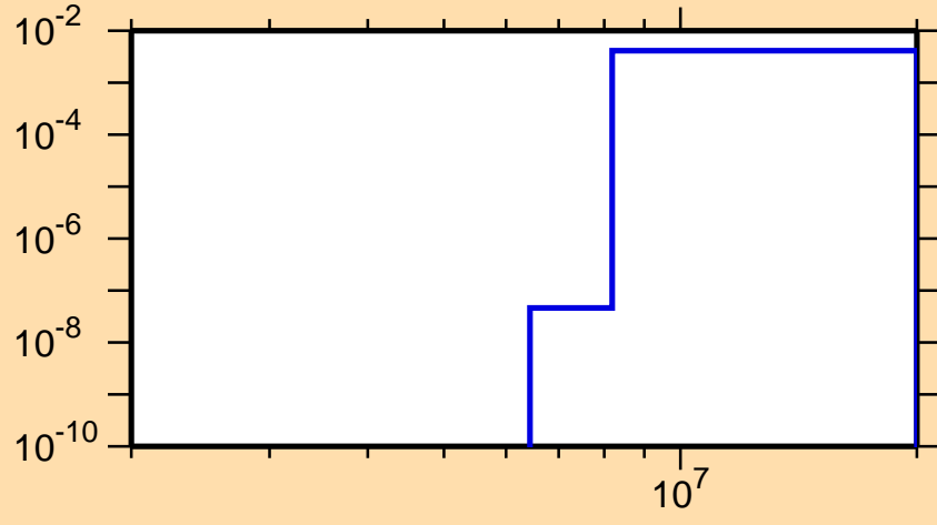
\sigma vs. E for ^{104}\text{Ru}(n,p)
