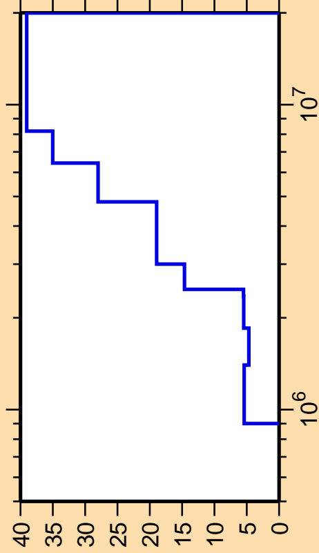
\Delta\sigma/\sigma vs. E for ^{104}\text{Ru}(n,n_4)
