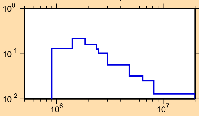
\sigma vs. E for ^{104}\text{Ru}(n,n_4)
