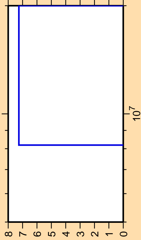
\Delta\sigma/\sigma vs. E for ^{104}\text{Ru}(n,nd)
