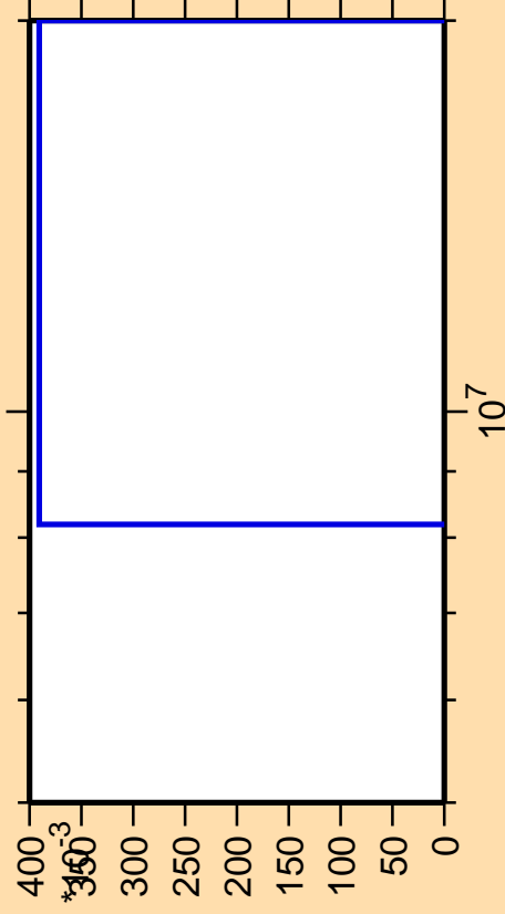
\Delta\sigma/\sigma vs. E for ^{104}\text{Ru}(n,nt)
