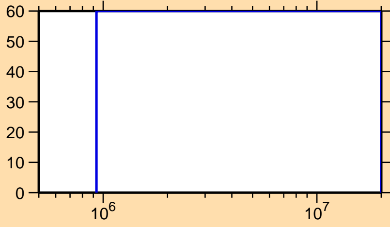
\Delta\sigma/\sigma vs. E for ^{105}\text{Ru}(n,\gamma)
