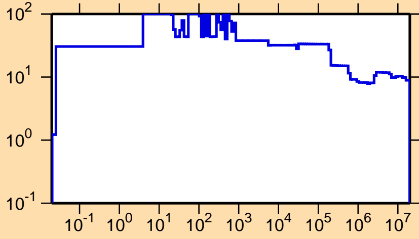
\Delta\sigma/\sigma vs. E for ^{105}\text{Ru}(n,\text{nonel.})
