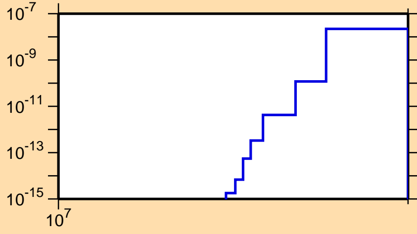
\sigma vs. E for ^{105}\text{Ru}(n,2n\alpha)
