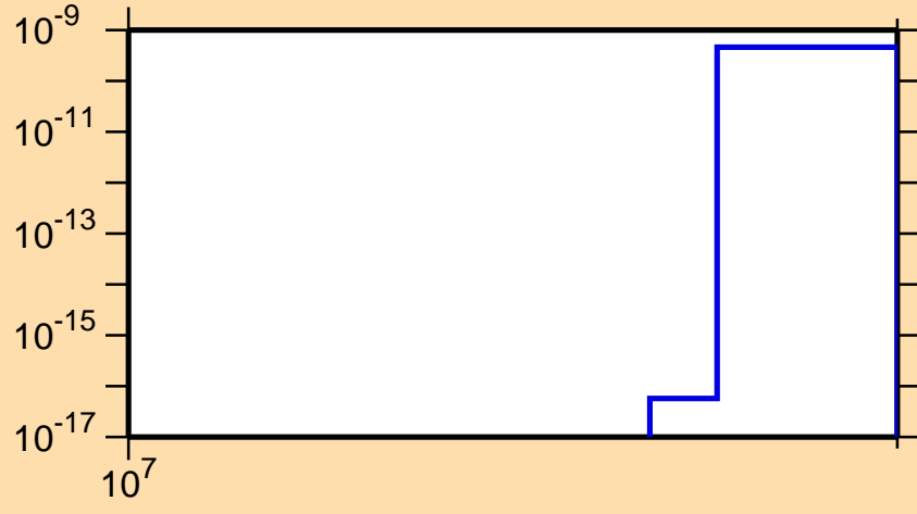
\sigma vs. E for ^{105}\text{Ru}(n,nt)
