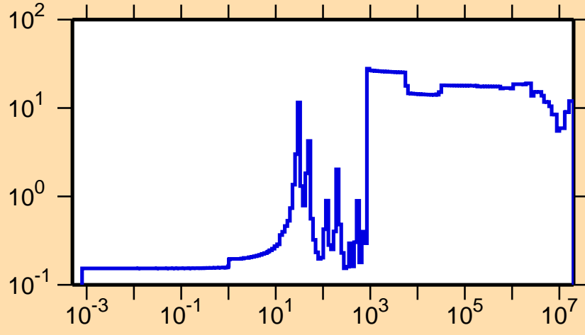
\Delta\sigma/\sigma vs. E for ^{105}\text{Ru}(n,\text{el.})
