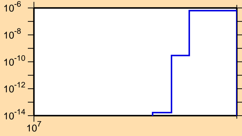
\sigma vs. E for ^{105}\text{Ru}(n,\text{nd})
