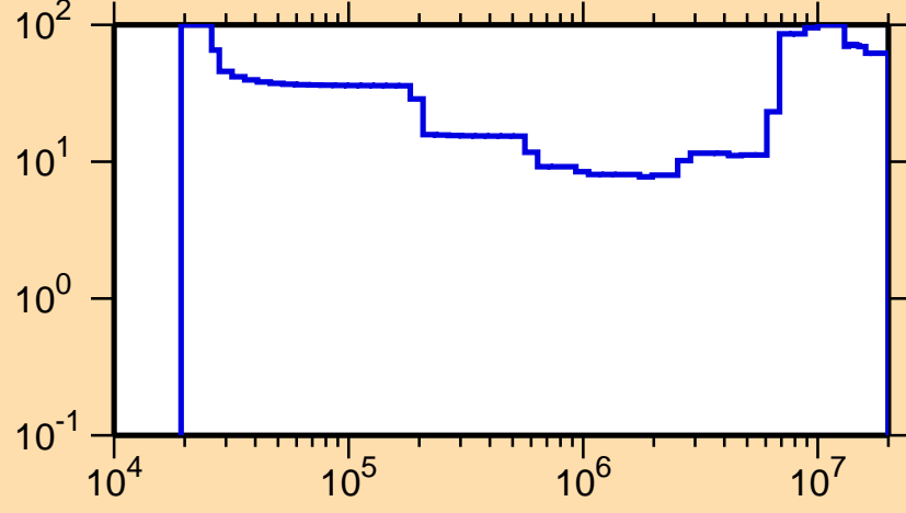
\Delta\sigma/\sigma vs. E for ^{105}\text{Ru}(n,\text{inel.})
