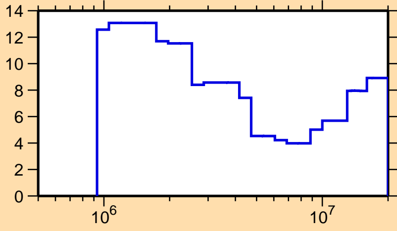
\Delta\sigma/\sigma vs. E for ^{105}\text{Ru}(n,\text{tot.})
