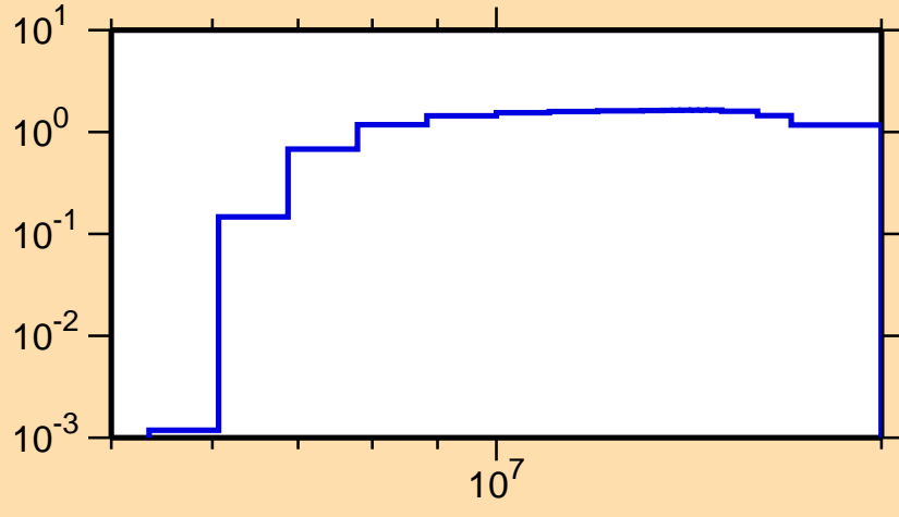
\sigma vs. E for ^{105}\text{Ru}(n,2n)
