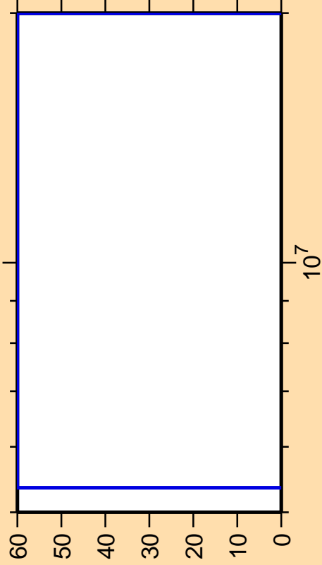
\Delta\sigma/\sigma vs. E for ^{105}\text{Ru}(n,p)
