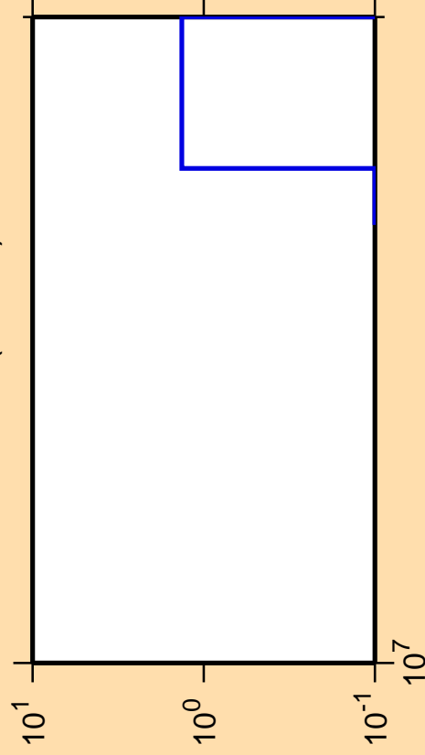
\Delta\sigma/\sigma vs. E for ^{105}\text{Ru}(n,\text{He3})
