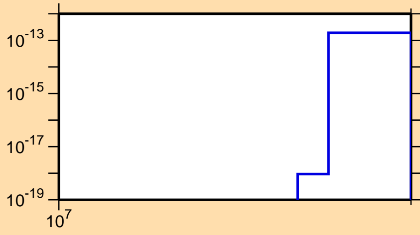
\sigma vs. E for ^{105}\text{Ru}(n,\text{He3})
