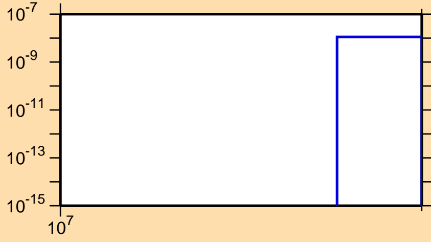
\sigma vs. E for ^{105}\text{Ru}(n,2np)
