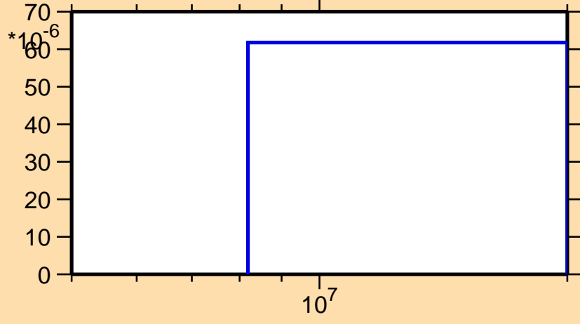
\sigma vs. E for ^{105}\text{Ru}(n,np)
