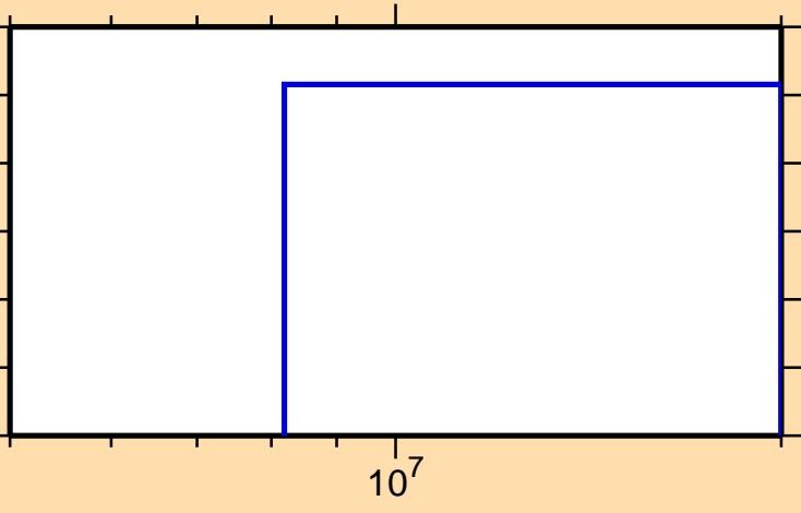
\sigma vs. E for ^{105}\text{Ru}(n,\text{nd})
