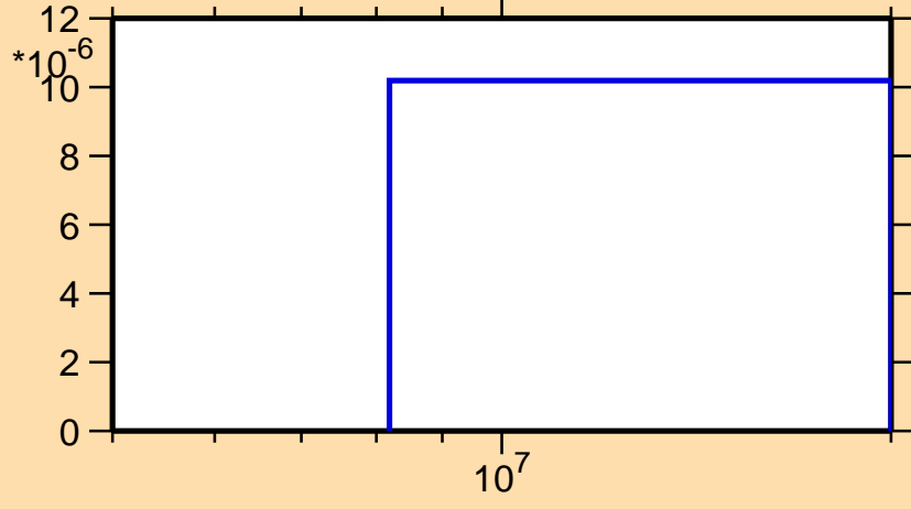
\sigma vs. E for ^{105}\text{Ru}(n,t)
