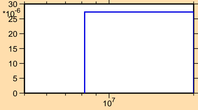
\sigma vs. E for ^{105}\text{Ru}(n,n\alpha)
