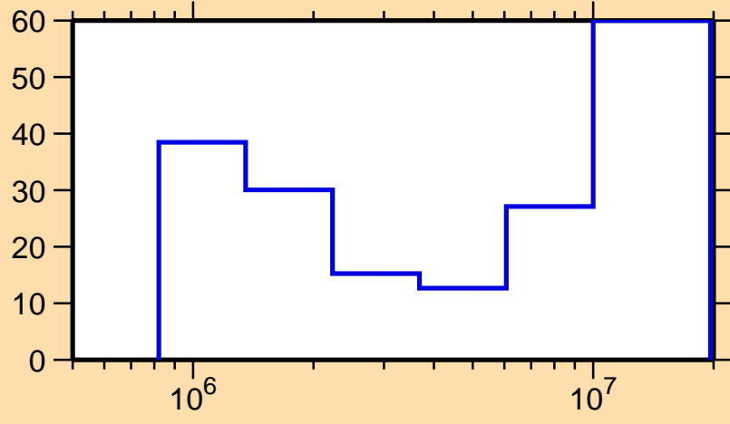
\Delta\sigma/\sigma vs. E for ^{107}\text{Ru}(n,n\text{cont.})
