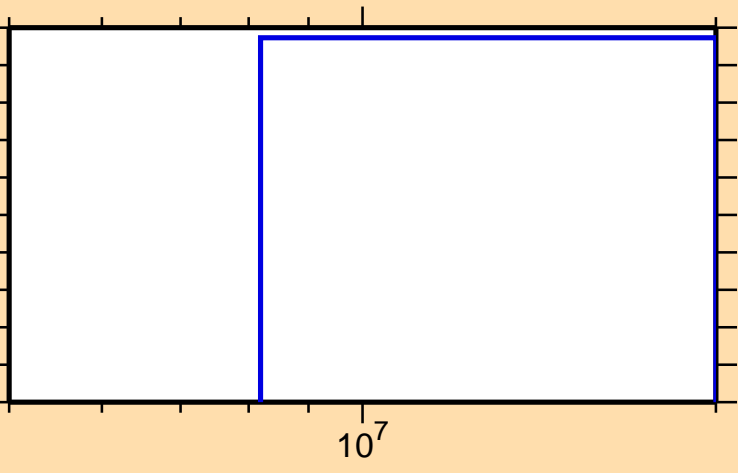
\sigma vs. E for ^{107}\text{Ru}(n,np)
