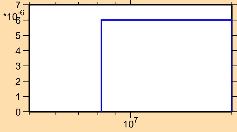
\sigma vs. E for ^{107}\text{Ru}(n,t)
