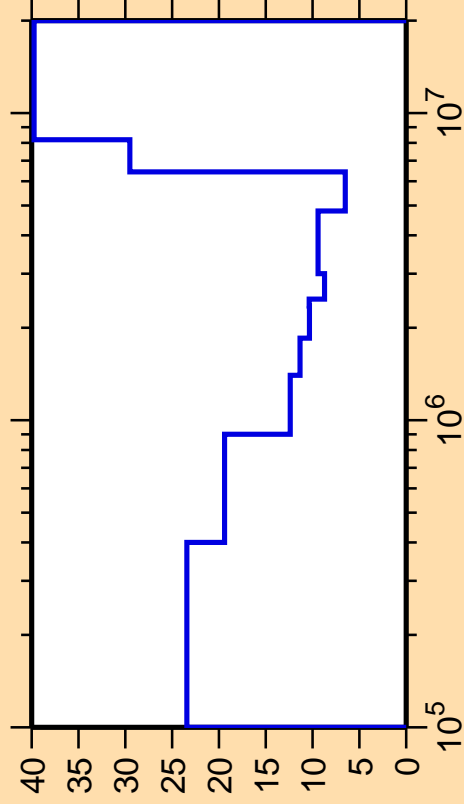
\Delta\sigma/\sigma vs. E for ^{107}\text{Ru}(n,\text{inel.})
