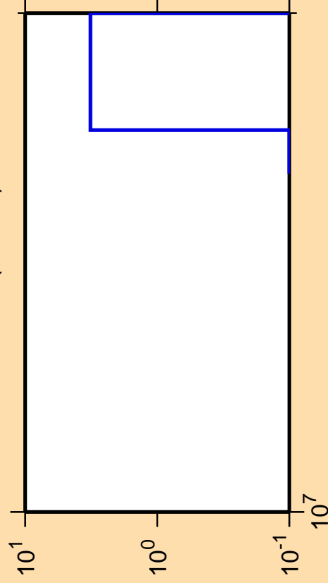
\Delta\sigma/\sigma vs. E for ^{108}\text{Ru}(n,2n\alpha)
