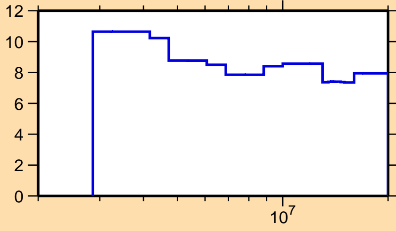
\Delta\sigma/\sigma vs. E for ^{108}\text{Ru}(n,n\text{onel.})
