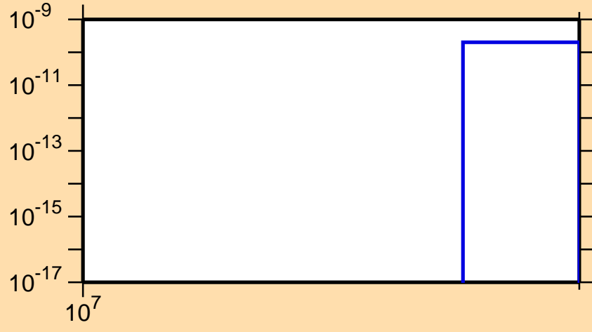
\sigma vs. E for ^{108}\text{Ru}(n,nt)
