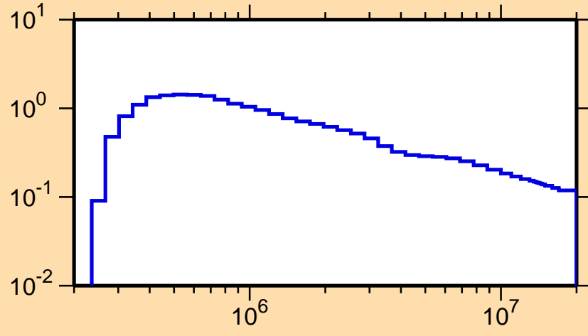
\sigma vs. E for ^{108}\text{Ru}(n,n_1)
