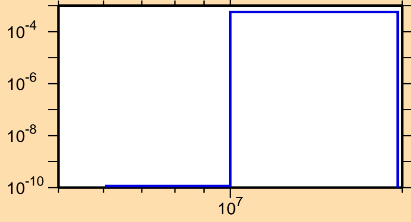
\sigma vs. E for ^{108}\text{Ru}(n,p)
