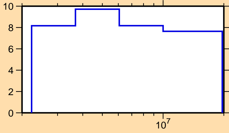
\Delta\sigma/\sigma vs. E for ^{108}\text{Ru}(n,n\text{onel.})
