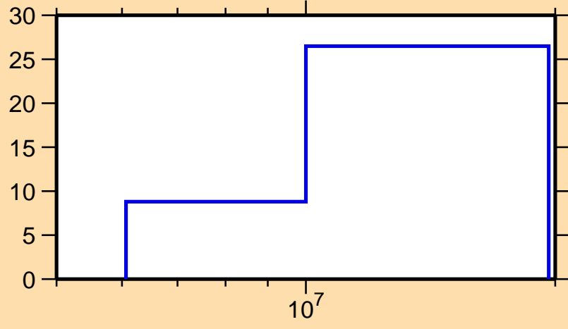
\Delta\sigma/\sigma vs. E for ^{108}\text{Ru}(n,\text{inel.})
