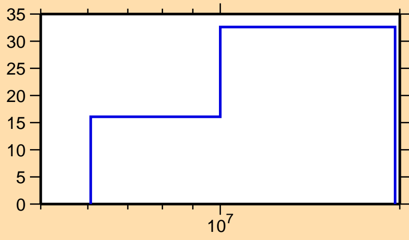
\Delta\sigma/\sigma vs. E for ^{108}\text{Ru}(n,n\text{cont.})
