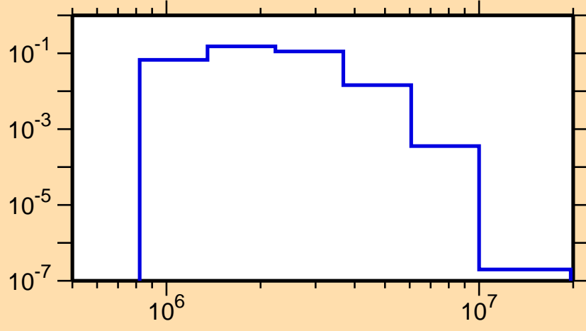
\sigma vs. E for ^{108}\text{Ru}(n,n_4)
