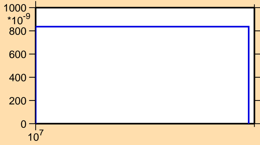
\sigma vs. E for ^{108}\text{Ru}(n,t)
