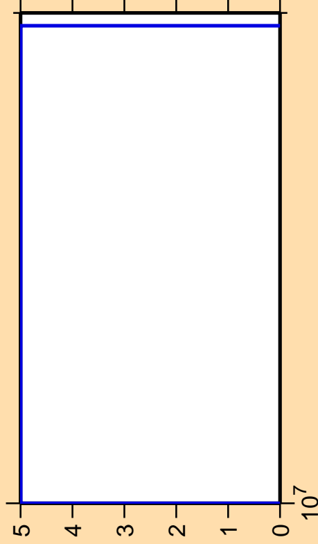
\Delta\sigma/\sigma vs. E for ^{108}\text{Ru}(n,nt)
