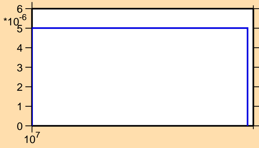
\sigma vs. E for ^{108}\text{Ru}(n,np)
