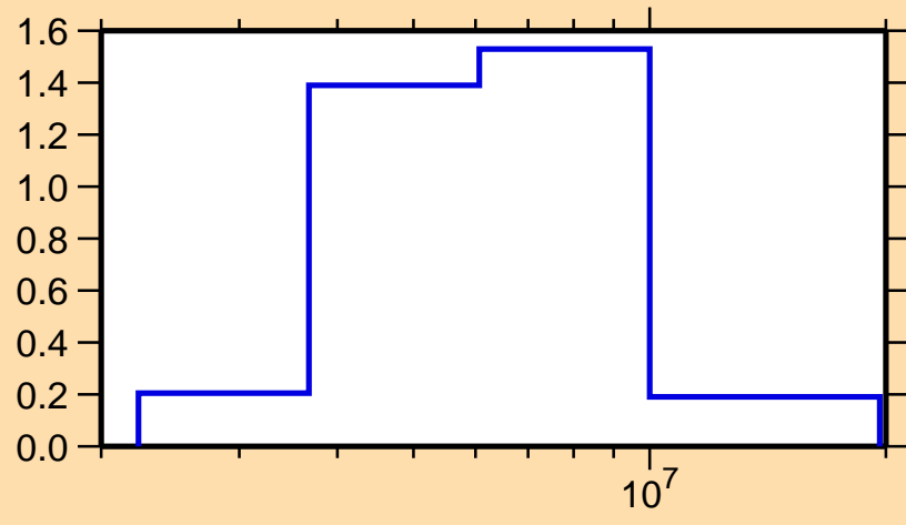
\sigma vs. E for ^{108}\text{Ru}(n,n\text{cont.})
