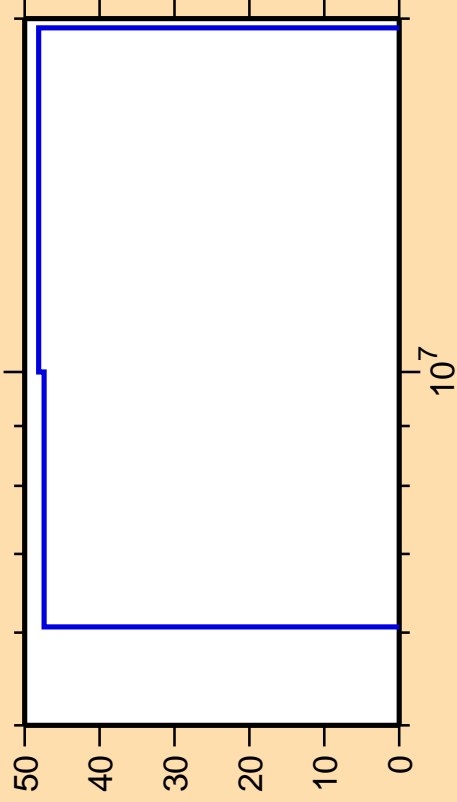
\Delta\sigma/\sigma vs. E for ^{108}\text{Ru}(n,p)
