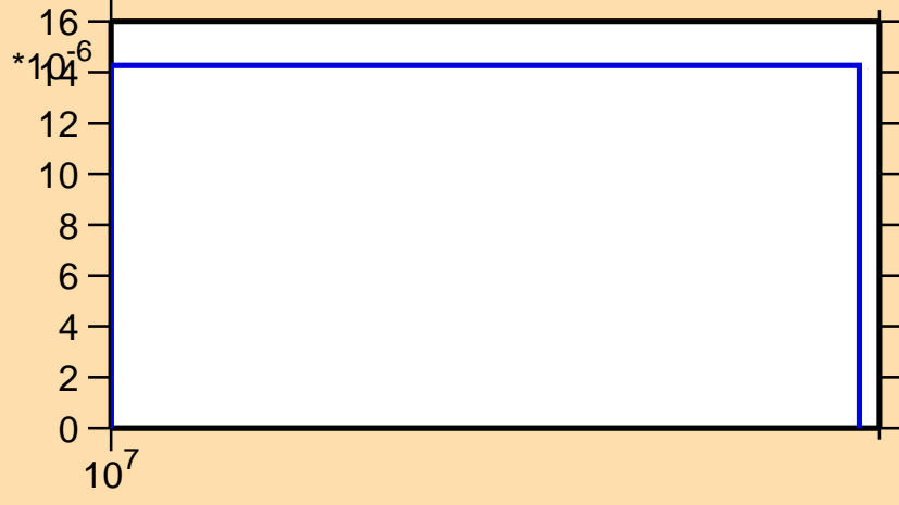
\sigma vs. E for ^{108}\text{Ru}(n,d)
