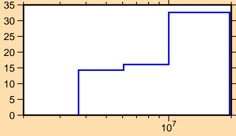
\Delta\sigma/\sigma vs. E for ^{108}\text{Ru}(n,n\text{cont.})
