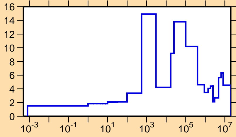
\Delta\sigma/\sigma vs. E for ^{108}\text{Ru}(n,\text{el.})
