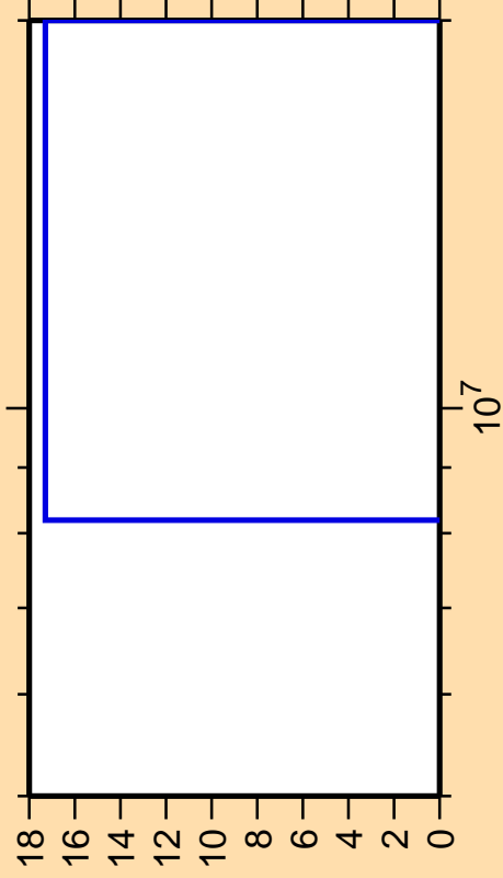
\Delta\sigma/\sigma vs. E for ^{108}\text{Ru}(n,3n)
