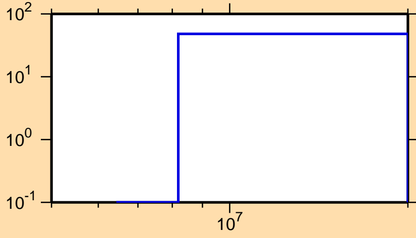
\Delta\sigma/\sigma vs. E for ^{108}\text{Ru}(n,p)
