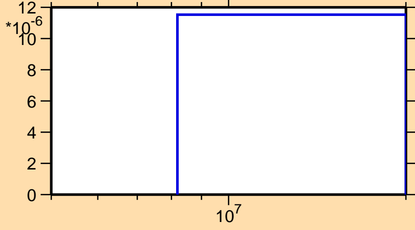
\sigma vs. E for ^{108}\text{Ru}(n,d)
