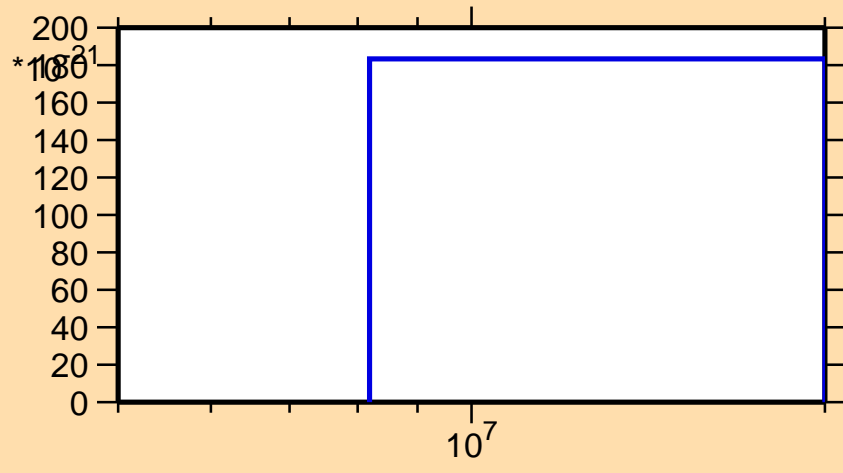
\sigma vs. E for ^{108}\text{Ru}(n,2np)
