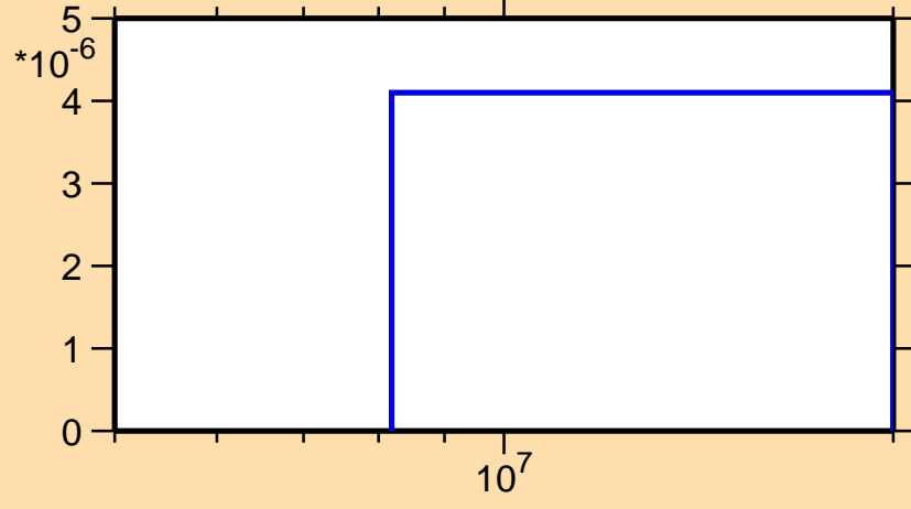
\sigma vs. E for ^{108}\text{Ru}(n,np)
