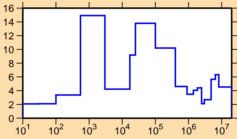
\Delta\sigma/\sigma vs. E for ^{108}\text{Ru}(n,\text{el.})
