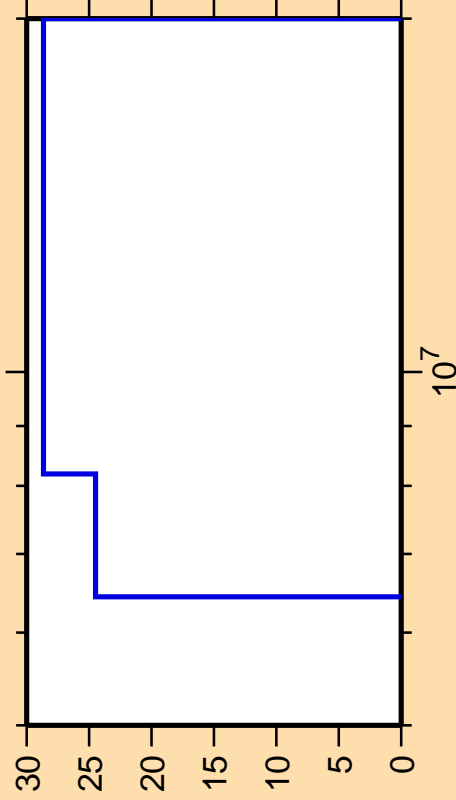
\Delta\sigma/\sigma vs. E for ^{108}\text{Ru}(n,n_1)
