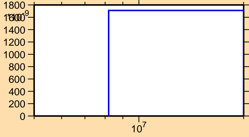
\sigma vs. E for ^{108}\text{Ru}(n,n\alpha)
