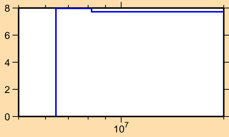
\Delta\sigma/\sigma vs. E for ^{108}\text{Ru}(n,\text{nonel.})
