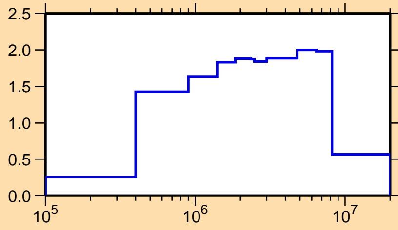
\sigma vs. E for ^{108}\text{Ru}(n,\text{inel.})
