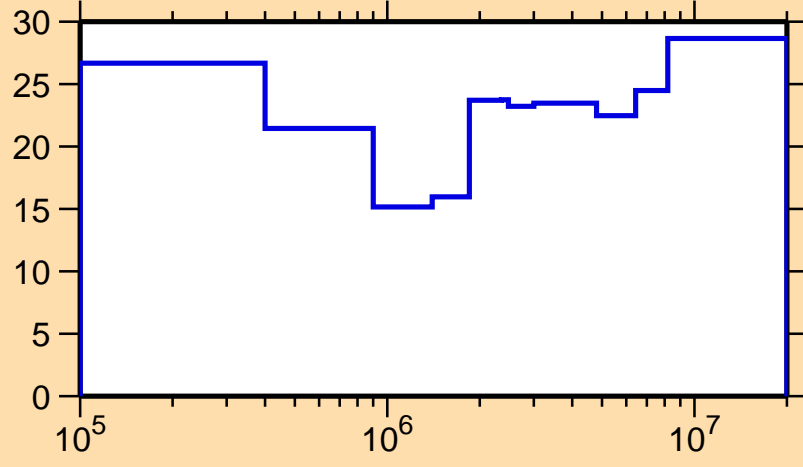
\Delta\sigma/\sigma vs. E for ^{108}\text{Ru}(n,n_1)
