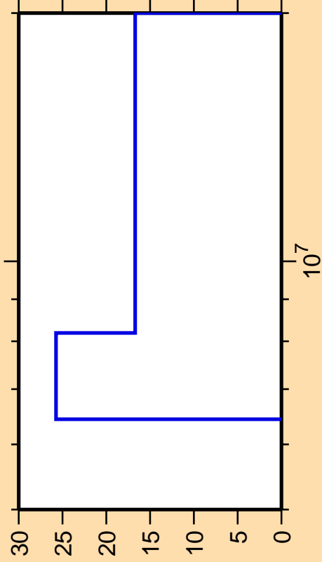
\Delta\sigma/\sigma vs. E for ^{108}\text{Ru}(n,2n)
