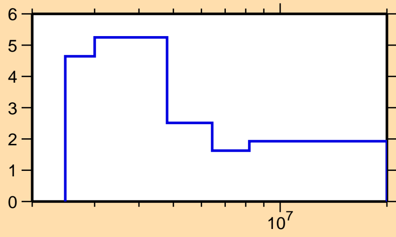
\Delta\sigma/\sigma vs. E for ^{108}\text{Ru}(n,\text{tot.})
