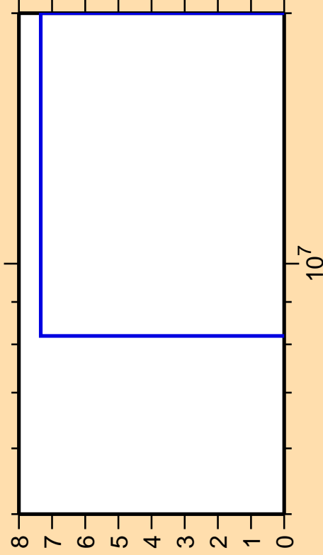
\Delta\sigma/\sigma vs. E for ^{108}\text{Ru}(n,nt)
