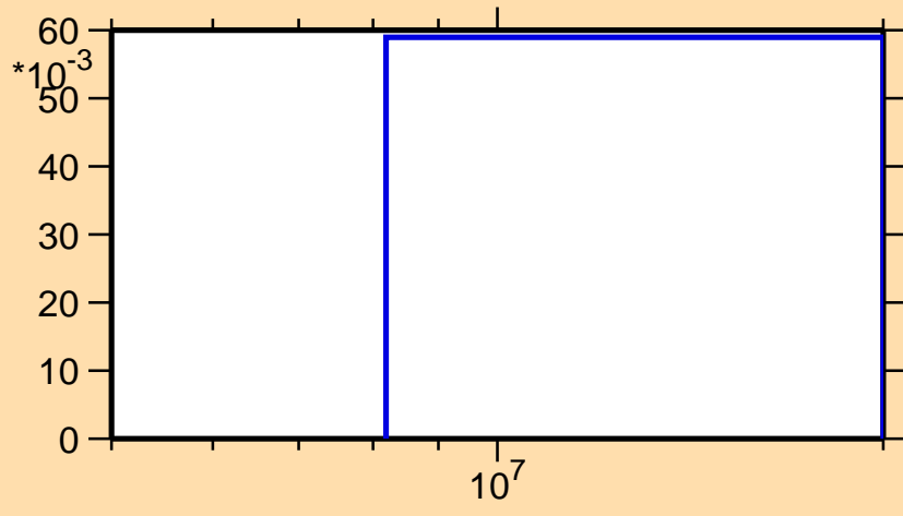
\sigma vs. E for ^{108}\text{Ru}(n,3n)
