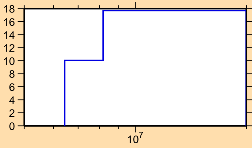
\Delta\sigma/\sigma vs. E for ^{108}\text{Ru}(n,\text{inel.})
