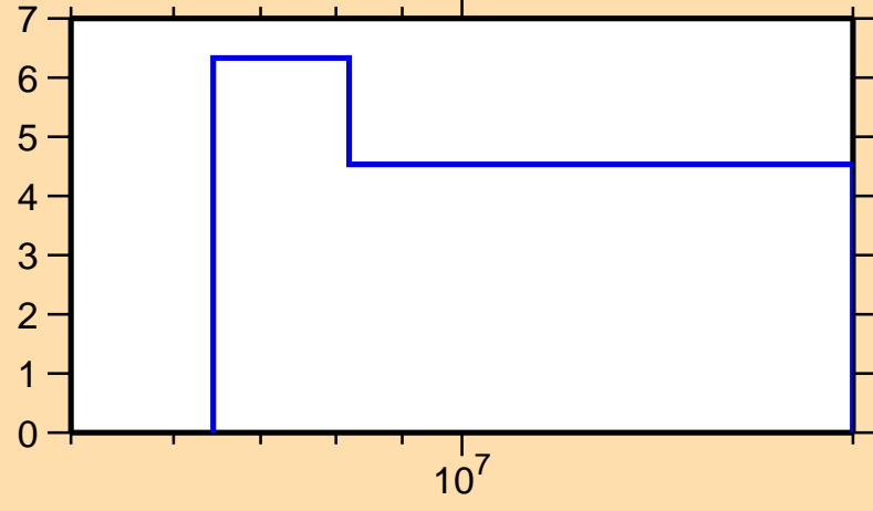
\Delta\sigma/\sigma vs. E for ^{108}\text{Ru}(n,\text{el.})
