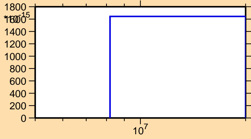
\sigma vs. E for ^{108}\text{Ru}(n,nt)
