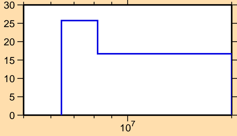
\Delta\sigma/\sigma vs. E for ^{108}\text{Ru}(n,2n)
