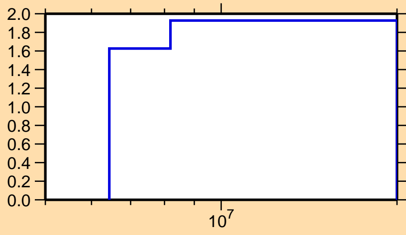
\Delta\sigma/\sigma vs. E for ^{108}\text{Ru}(n,\text{tot.})
