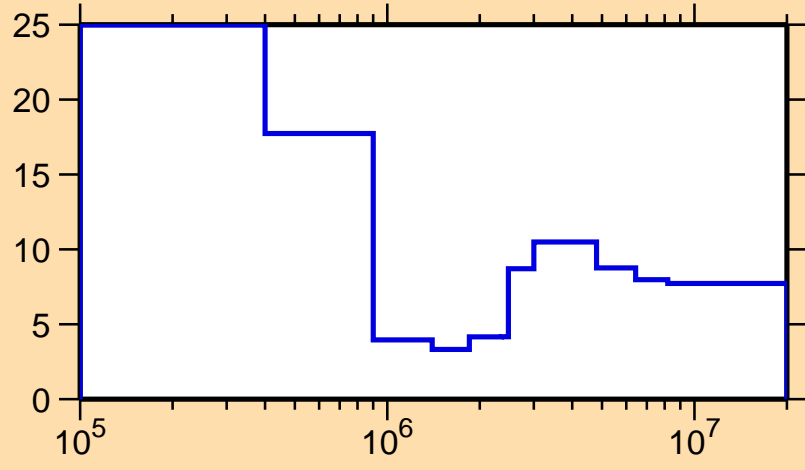
\Delta\sigma/\sigma vs. E for ^{108}\text{Ru}(n,\text{nonel.})
