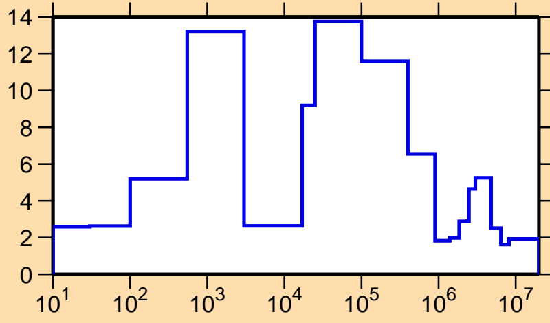
\Delta\sigma/\sigma vs. E for ^{108}\text{Ru}(n,\text{tot.})
