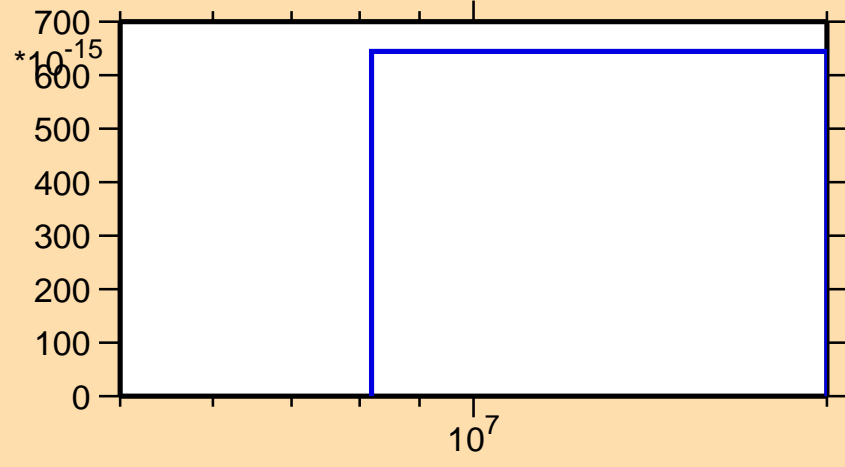
\sigma vs. E for ^{108}\text{Ru}(n,\text{nd})
