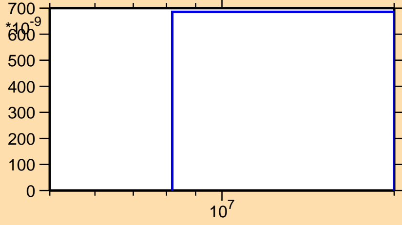
\sigma vs. E for ^{108}\text{Ru}(n,t)
