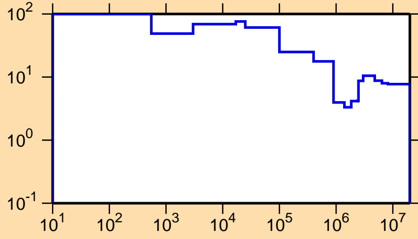
\Delta\sigma/\sigma vs. E for ^{108}\text{Ru}(n,\text{nonel.})
