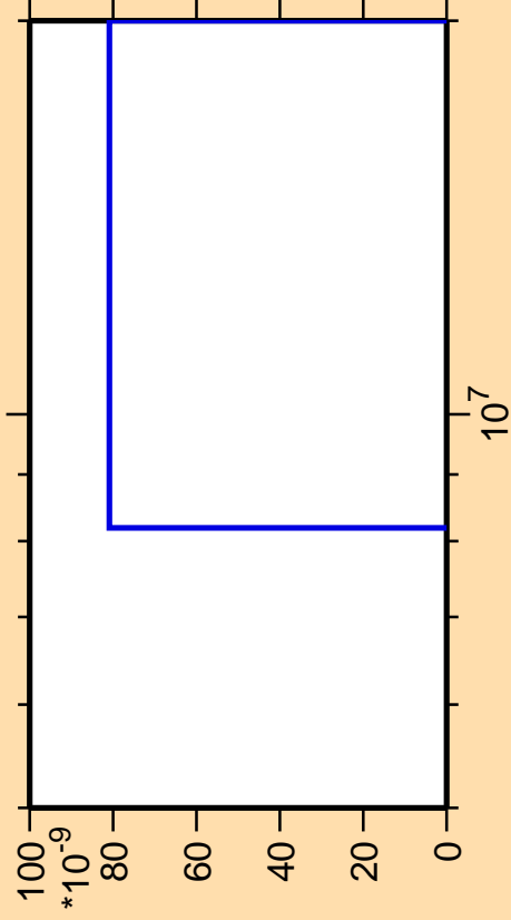
\Delta\sigma/\sigma vs. E for ^{108}\text{Ru}(n,2np)
