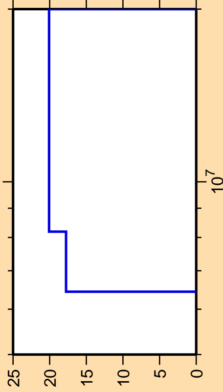
\Delta\sigma/\sigma vs. E for ^{108}\text{Ru}(n,n\text{cont.})
