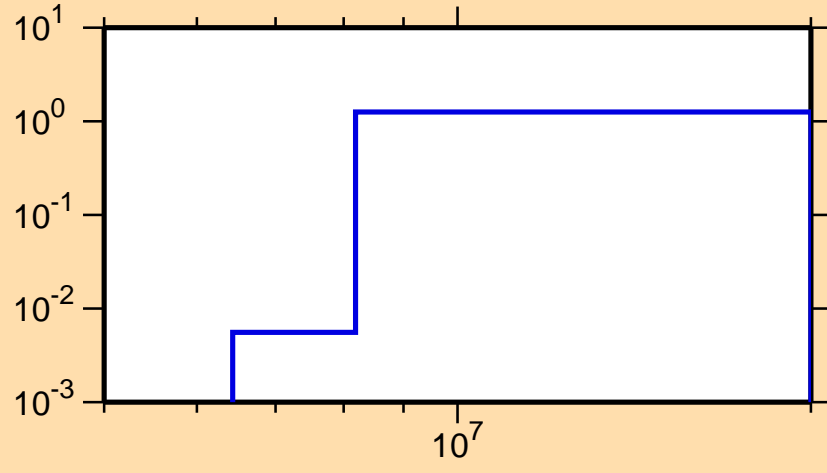
\sigma vs. E for ^{108}\text{Ru}(n,2n)
