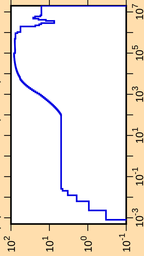
\Delta\mu/\mu vs. E for ^{109}\text{Ru}(\text{mt251})
