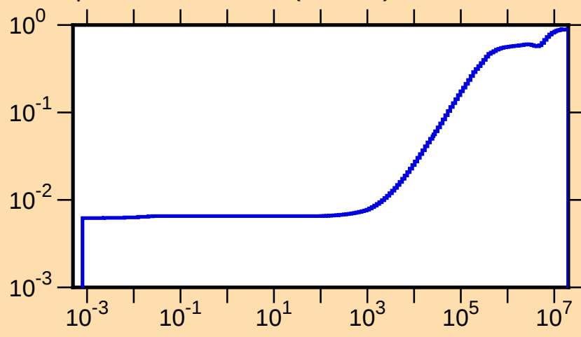
\mu vs. E for ^{109}\text{Ru}(\text{mt251})
