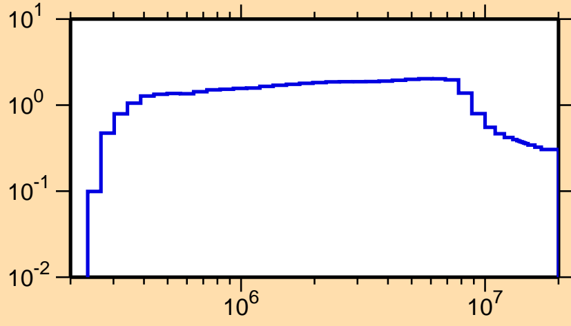
\sigma vs. E for ^{110}\text{Ru}(n,\text{inel.})
