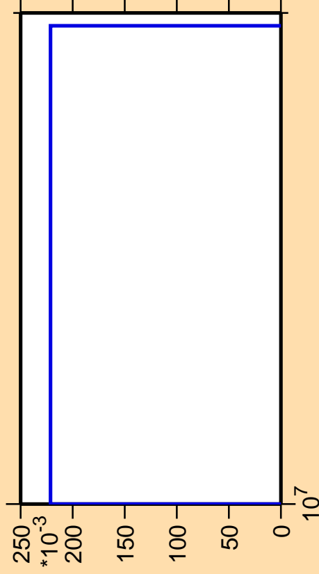
\Delta\sigma/\sigma vs. E for ^{110}\text{Ru}(n,\text{nd})
