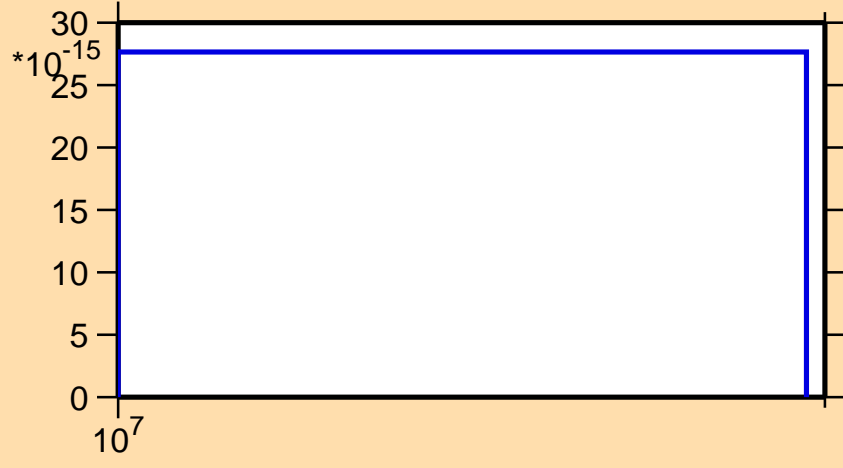
\sigma vs. E for ^{110}\text{Ru}(n,\text{nd})
