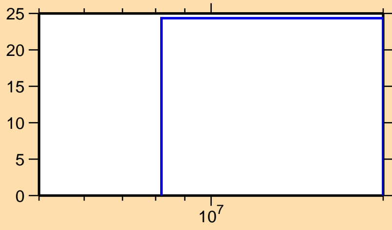
\Delta\sigma/\sigma vs. E for ^{110}\text{Ru}(n,el.)
