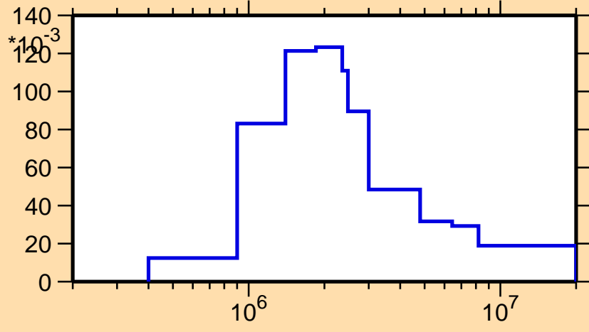
\sigma vs. E for ^{110}\text{Ru}(n,n_3)
