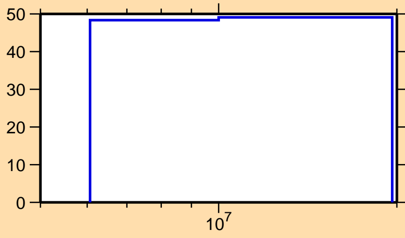
\Delta\sigma/\sigma vs. E for ^{111}\text{Ru}(n,ncont.)
