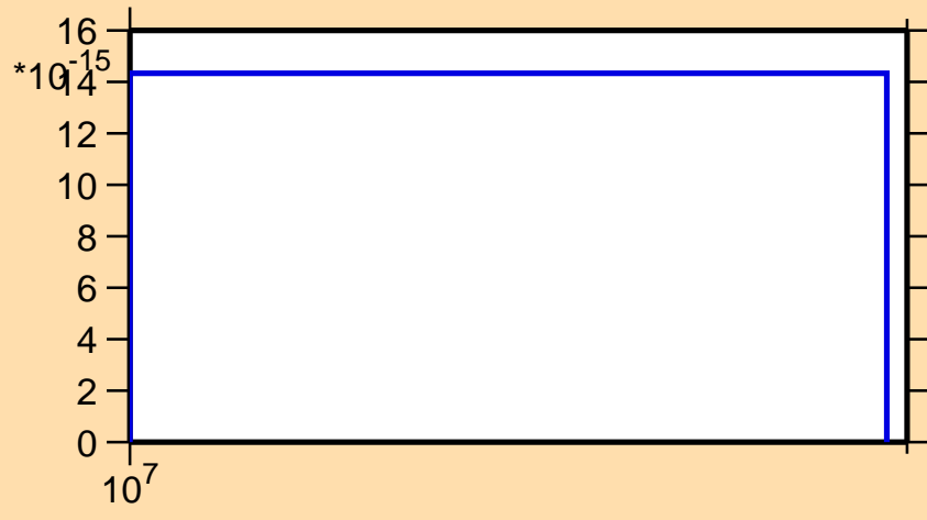
\sigma vs. E for ^{111}\text{Ru}(n,2np)
