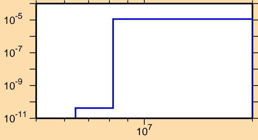
\sigma vs. E for ^{111}\text{Ru}(n,\alpha)
