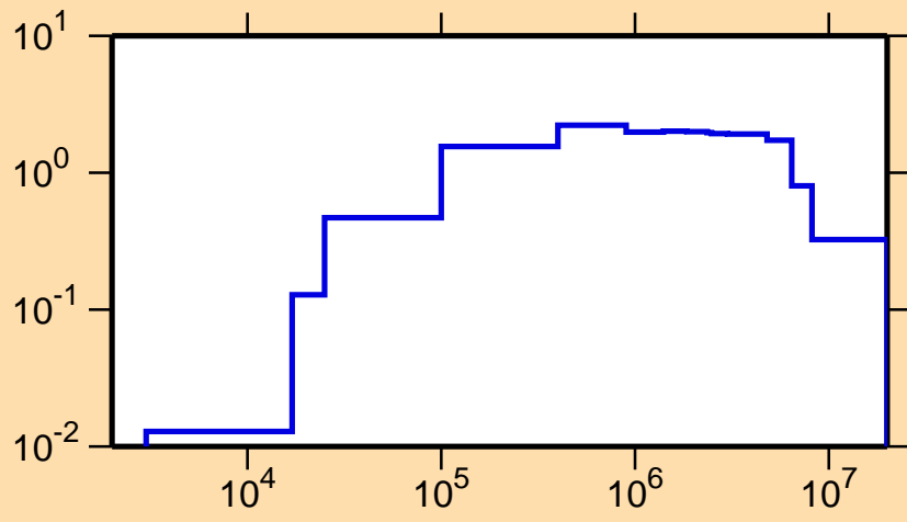
\sigma vs. E for ^{111}\text{Ru}(n,\text{inel.})
