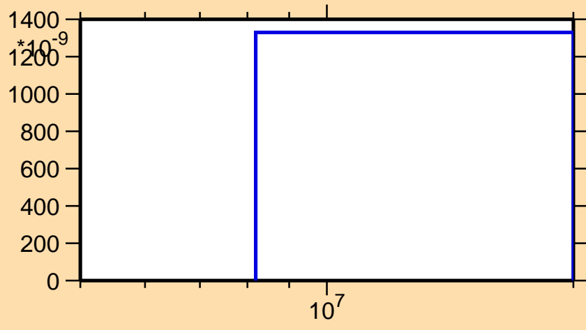
\sigma vs. E for ^{111}\text{Ru}(n,t)
