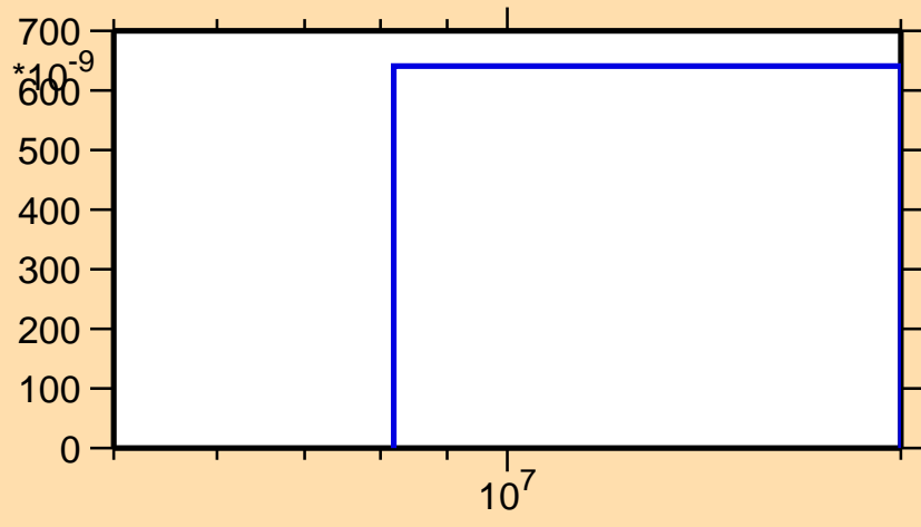
\sigma vs. E for ^{111}\text{Ru}(n,np)
