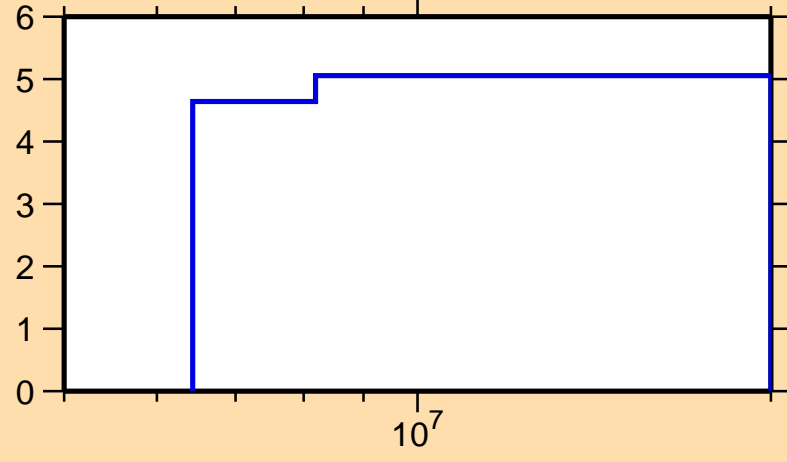
\Delta\sigma/\sigma vs. E for ^{111}\text{Ru}(n,\text{tot.})
