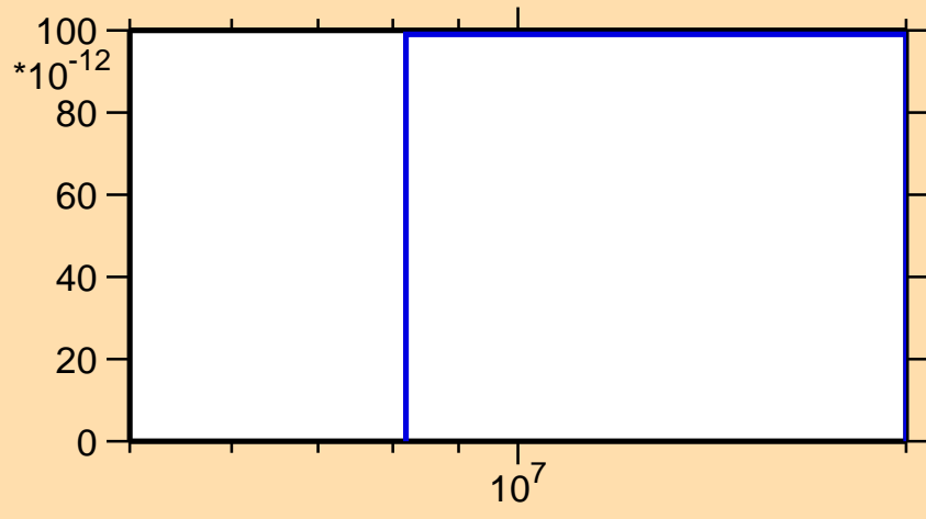
\sigma vs. E for ^{111}\text{Ru}(n,nd)
