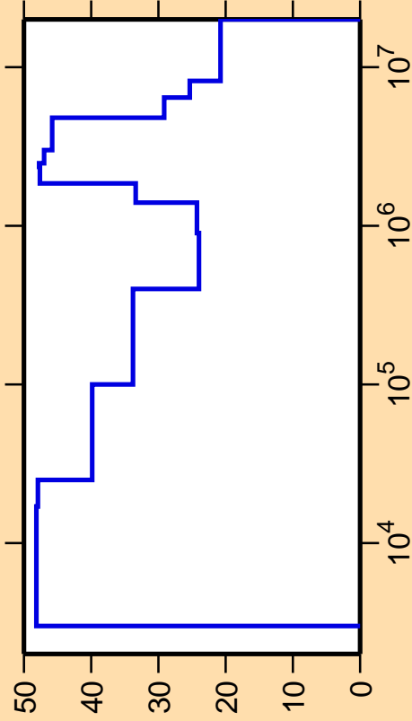
\Delta\sigma/\sigma vs. E for ^{111}\text{Ru}(n,n_1)
