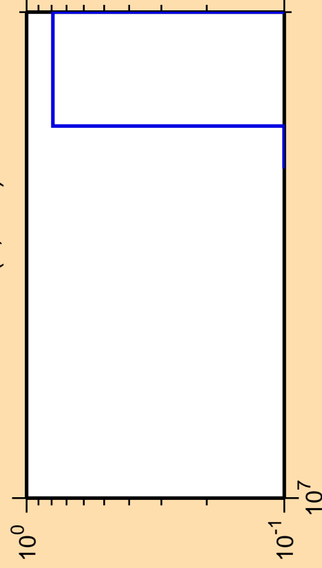
\Delta\sigma/\sigma vs. E for ^{112}\text{Ru}(n,2n\alpha)
