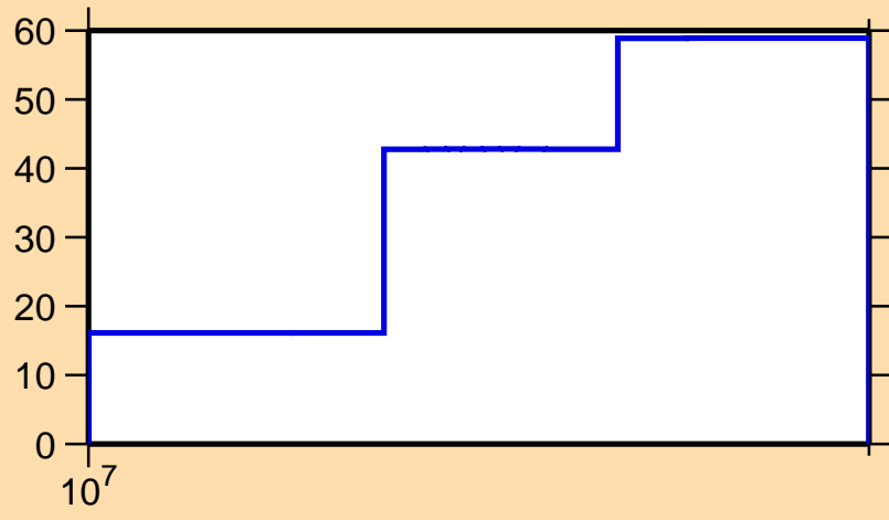
\Delta\sigma/\sigma vs. E for ^{112}\text{Ru}(n,2n)
