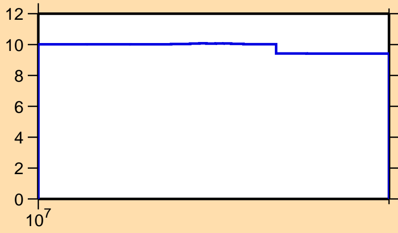
\Delta\sigma/\sigma vs. E for ^{112}\text{Ru}(n,\text{nonel.})
