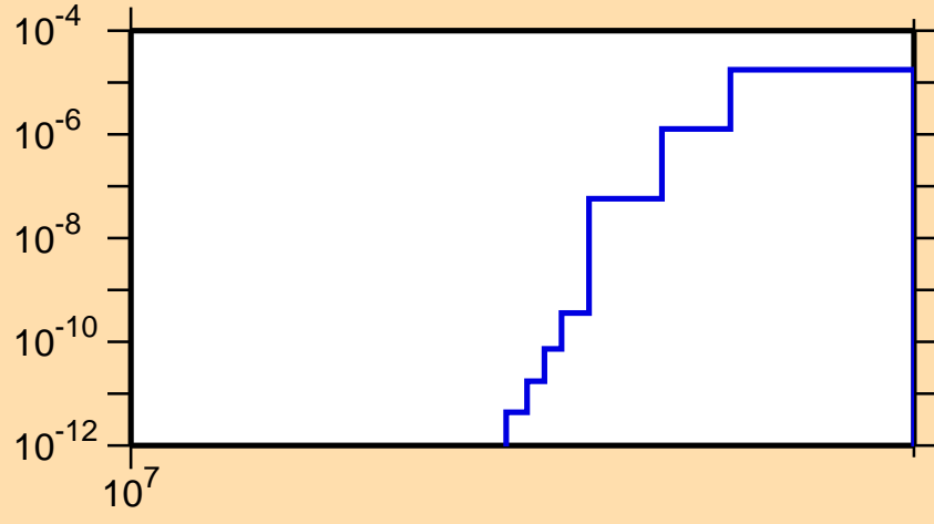
\sigma vs. E for ^{112}\text{Ru}(n,t)
