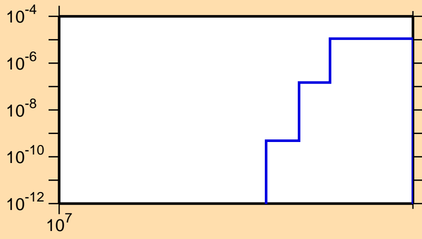
\sigma vs. E for ^{112}\text{Ru}(n,np)
