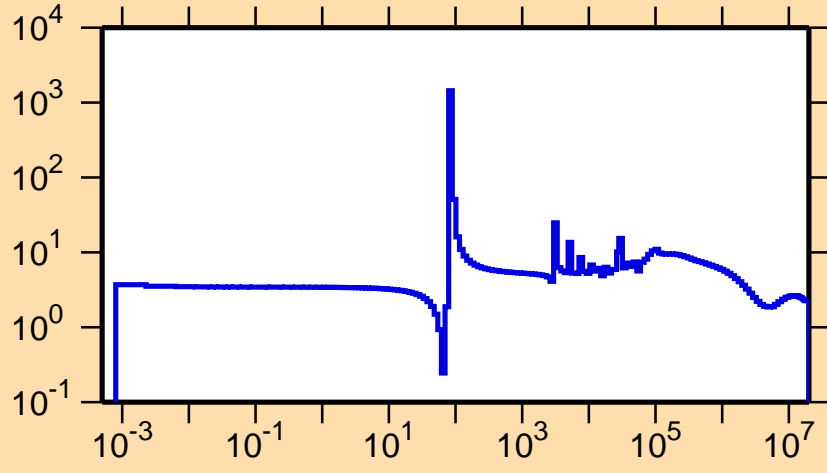
\sigma vs. E for ^{112}\text{Ru}(n,\text{el.})
