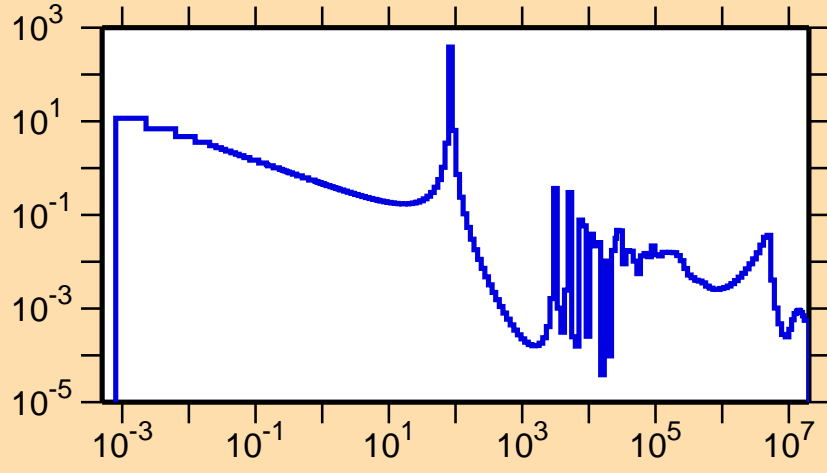
\sigma vs. E for ^{112}\text{Ru}(n,\gamma)
