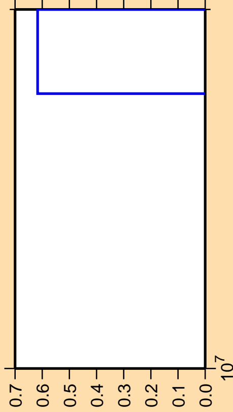
\Delta\sigma/\sigma vs. E for ^{112}\text{Ru}(n,\text{nd})
