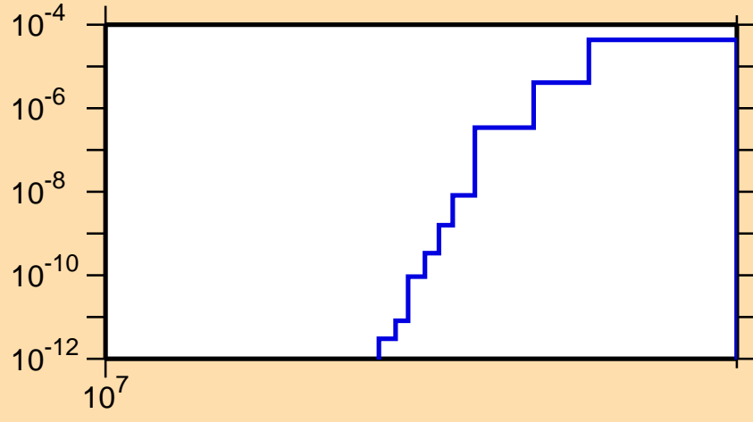
\sigma vs. E for ^{112}\text{Ru}(n,d)
