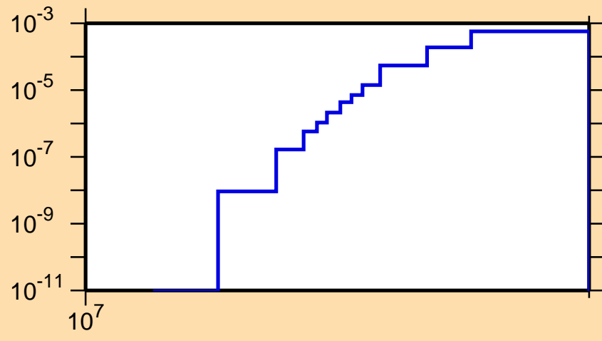
\sigma vs. E for ^{112}\text{Ru}(n,p)
