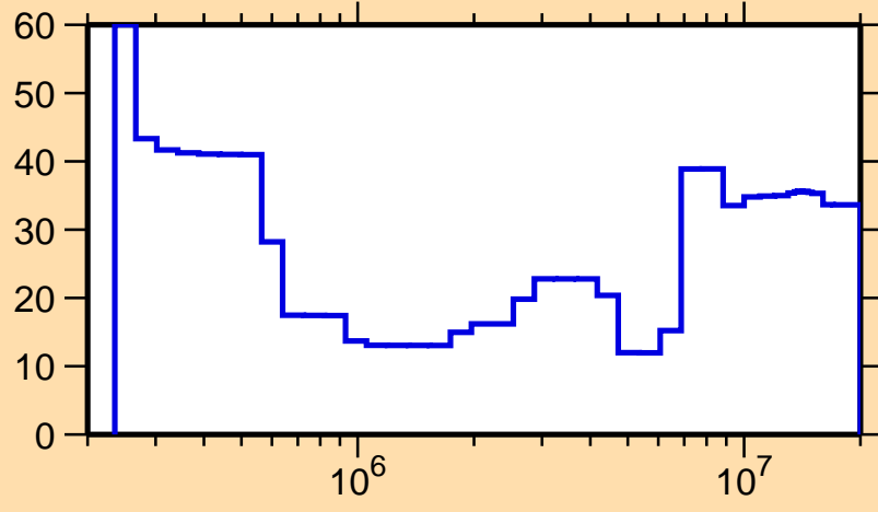
\Delta\sigma/\sigma vs. E for ^{112}\text{Ru}(n,\text{inel.})
