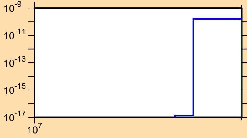
\sigma vs. E for ^{112}\text{Ru}(n,nt)
