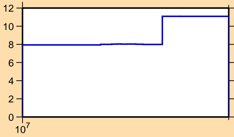
\Delta\sigma/\sigma vs. E for ^{112}\text{Ru}(n,\text{el.})
