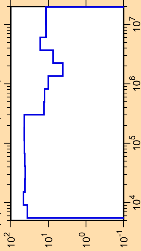
\Delta\mu/\mu vs. E for ^{112}\text{Ru}(\text{mt251})
