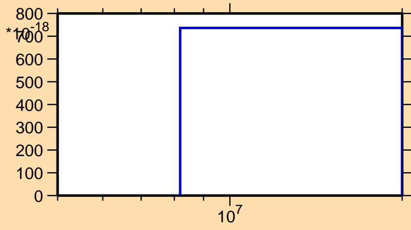
\sigma vs. E for ^{112}\text{Ru}(n,nd)
