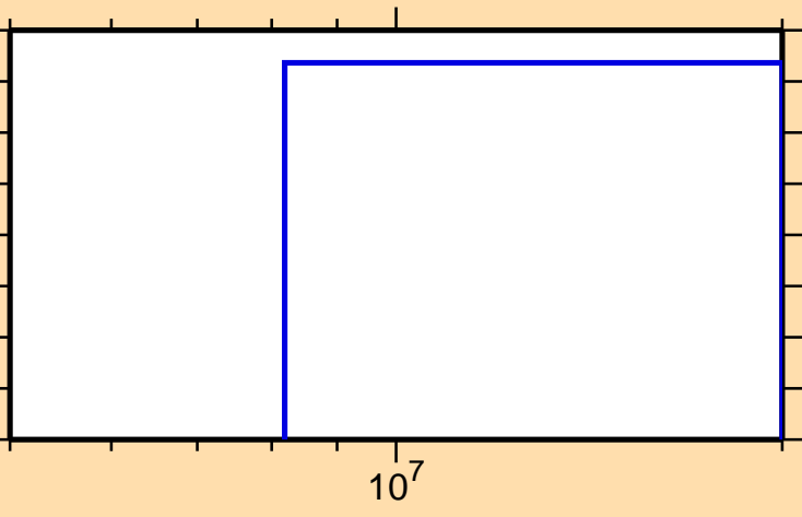
\sigma vs. E for ^{112}\text{Ru}(n,nd)
