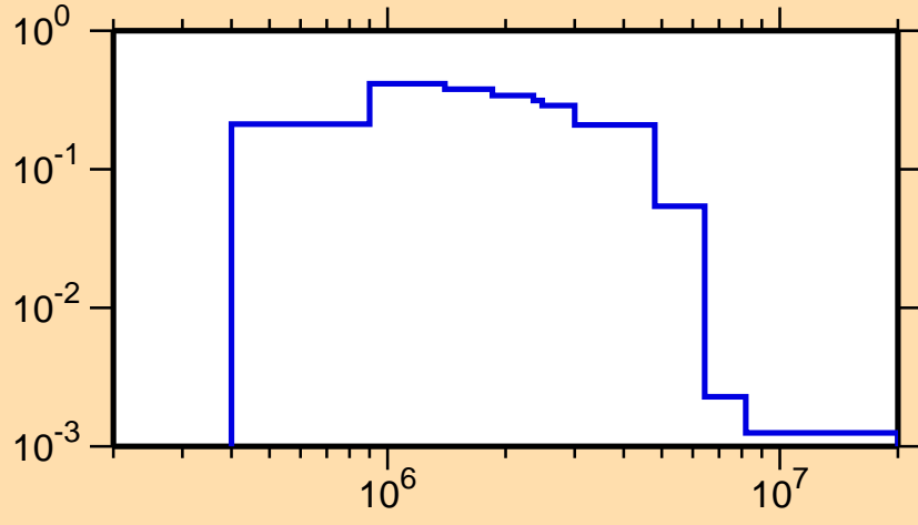
\sigma vs. E for ^{112}\text{Ru}(n,n_2)
