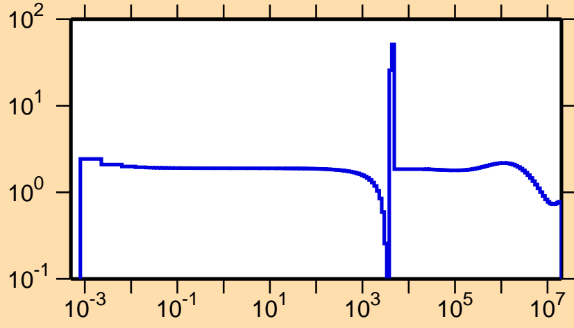
\sigma vs. E for ^{30}\text{S}(n,\text{el.})
