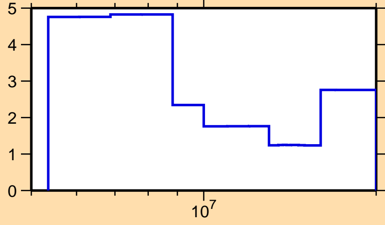
\Delta\sigma/\sigma vs. E for ^{30}\text{S}(n,el.)
