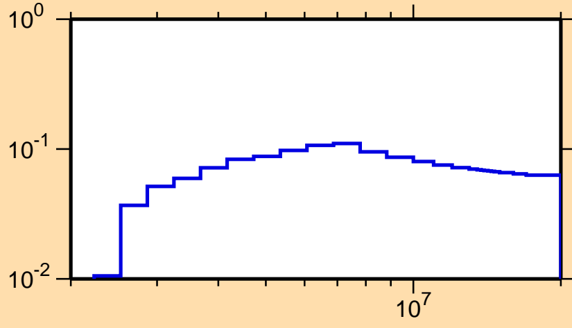
\sigma vs. E for ^{30}\text{S}(n,\text{inel.})
