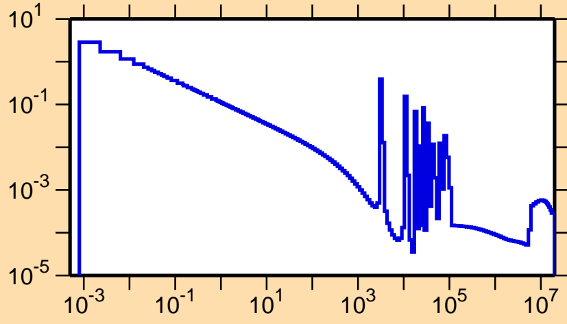
\sigma vs. E for ^{31}\text{S}(n,\gamma)
