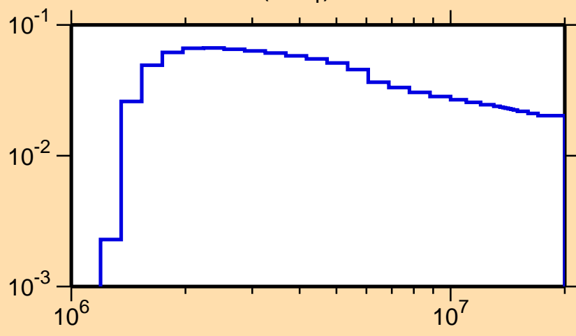
\sigma vs. E for ^{31}\text{S}(n,n_1)
