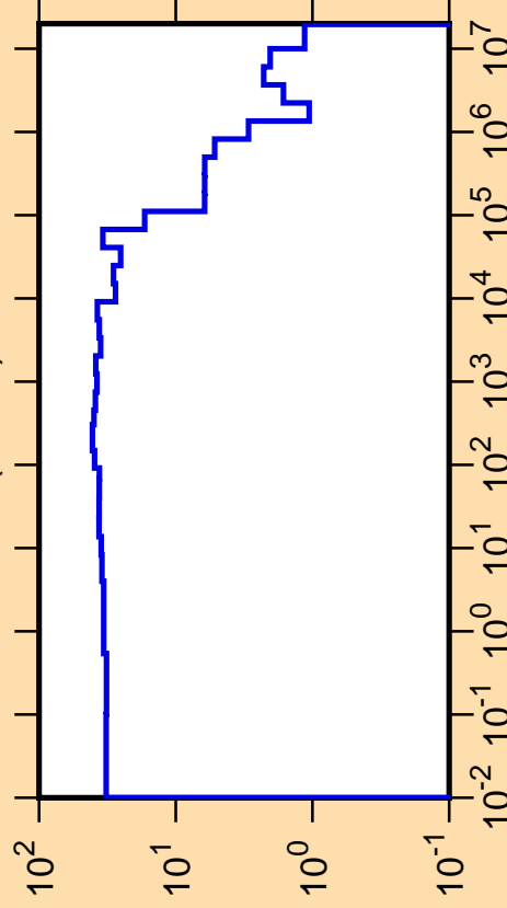
\Delta\sigma/\sigma vs. E for ^{31}\text{S}(n,\text{tot.})
