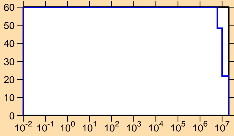
\Delta\sigma/\sigma vs. E for ^{31}\text{S}(n,\gamma)
