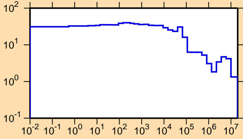
\Delta\sigma/\sigma vs. E for ^{31}\text{S}(n,el.)
