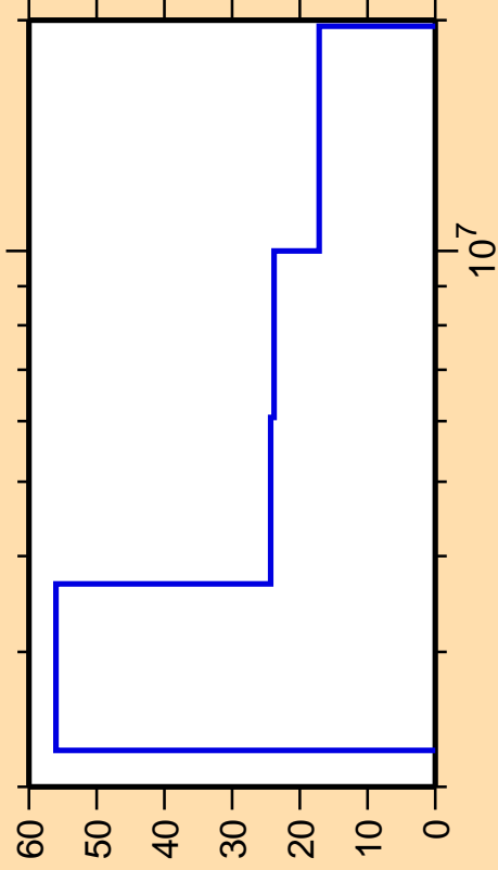
\Delta\sigma/\sigma vs. E for ^{31}\text{S}(n,\text{ncont.})
