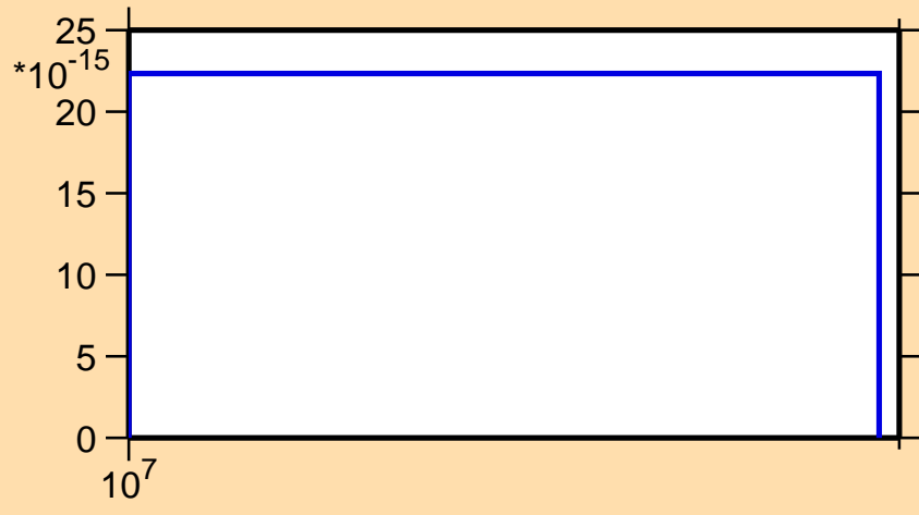
\sigma vs. E for ^{31}\text{S} (mt 45)
