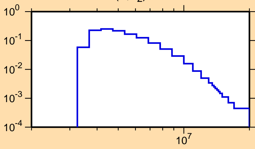
\sigma vs. E for ^{34}\text{S}(n,n_2)
