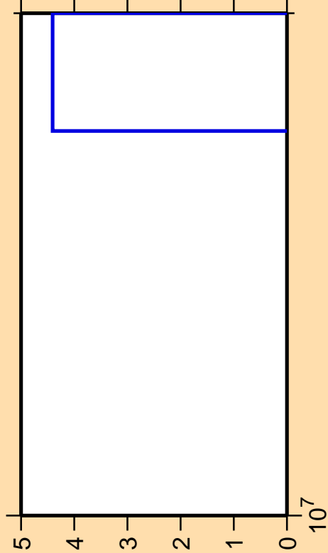
\Delta\sigma/\sigma vs. E for ^{34}\text{S}(n,pd)
