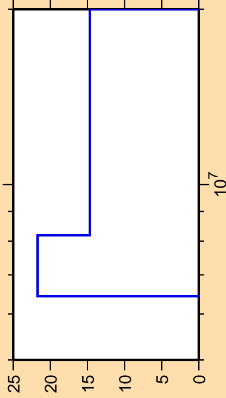
\Delta\sigma/\sigma vs. E for ^{34}\text{S}(n,\text{ncont.})
