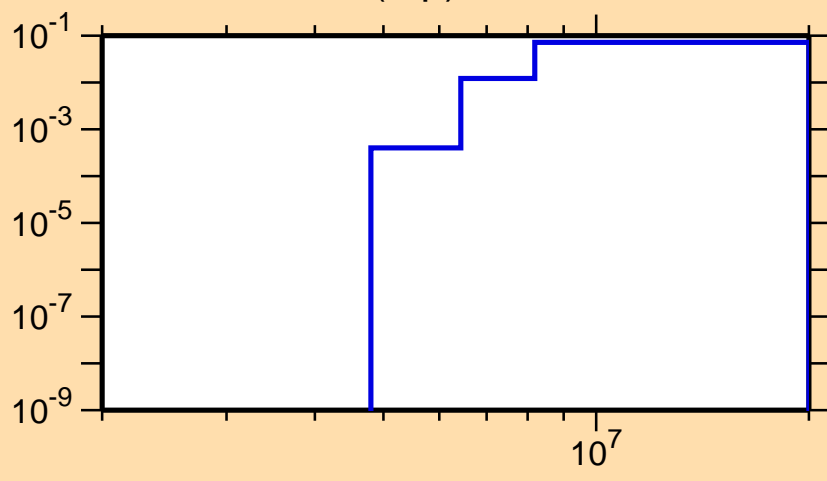
\sigma vs. E for ^{34}\text{S}(n,p)
