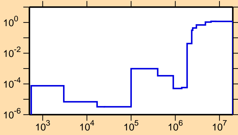
\sigma vs. E for ^{34}\text{S}(n,\text{nonel.})
