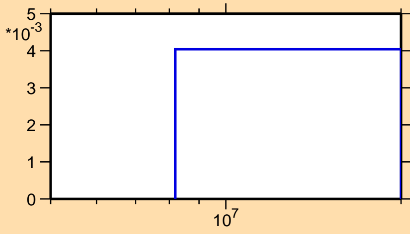
\sigma vs. E for ^{34}\text{S}(n,d)
