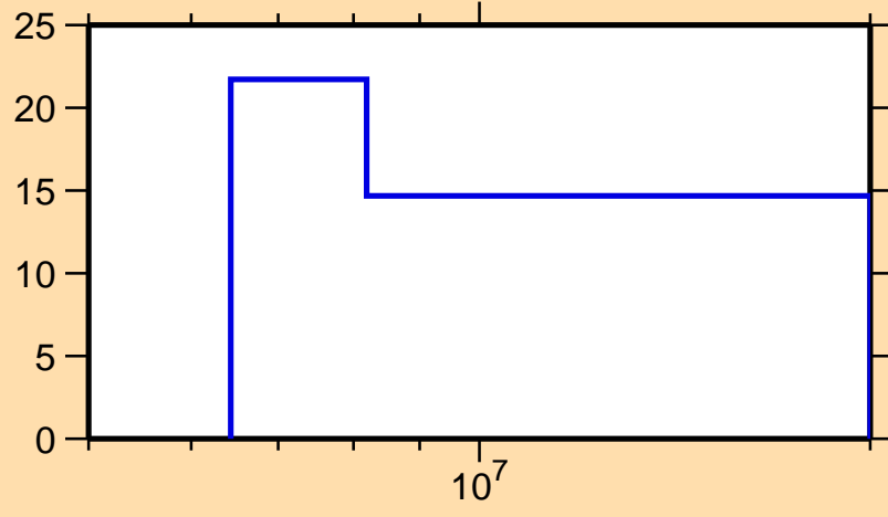
\Delta\sigma/\sigma vs. E for ^{34}\text{S}(n,ncont.)
