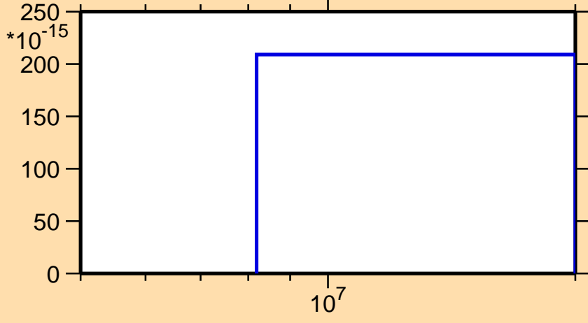
\sigma vs. E for ^{34}\text{S}(n,\text{nd})
