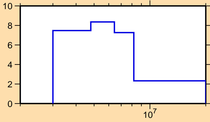
\Delta\sigma/\sigma vs. E for ^{34}\text{S}(n,el.)
