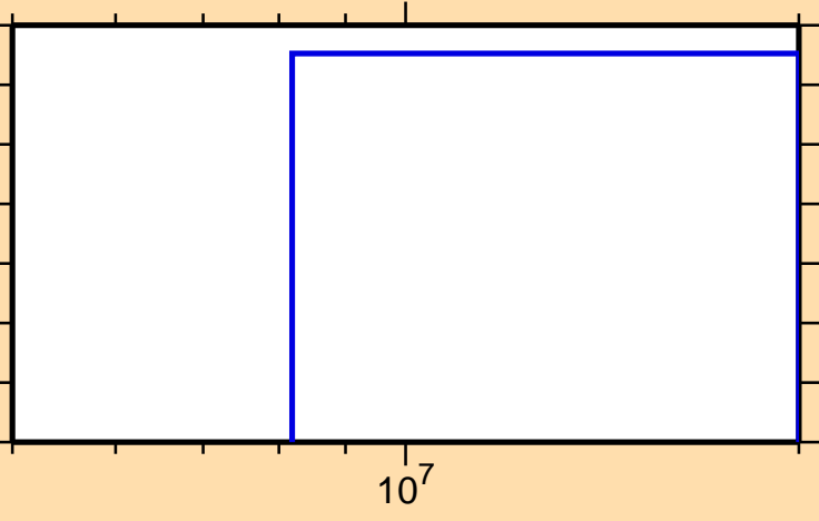
\sigma vs. E for ^{34}\text{S}(n,\text{He}3)
