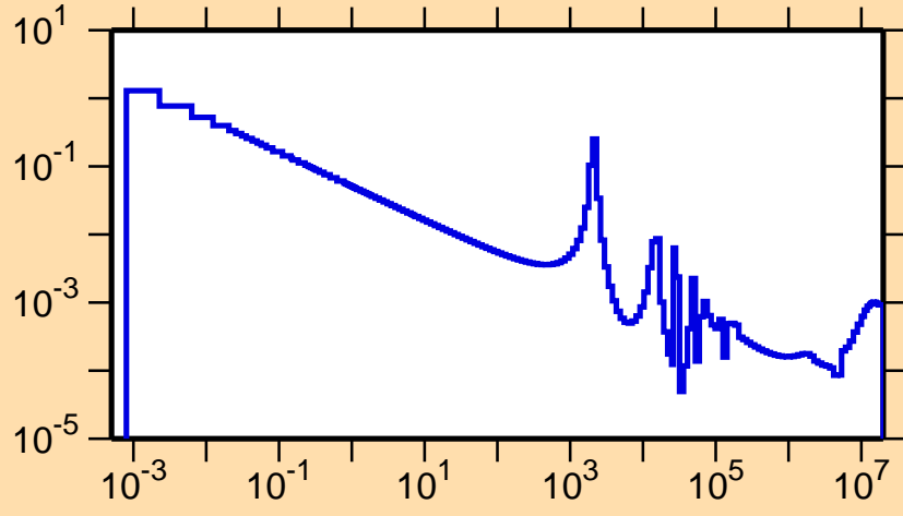
\sigma vs. E for ^{35}\text{S}(n,\gamma)
