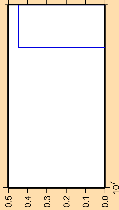
\Delta\sigma/\sigma vs. E for ^{35}\text{S}(n,\text{pt})
