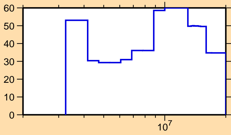
\Delta\sigma/\sigma vs. E for ^{35}\text{S}(n,p)
