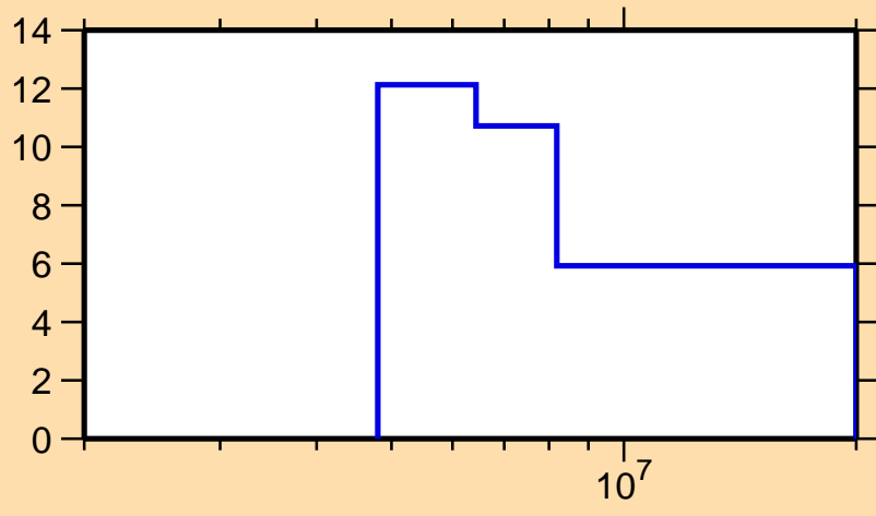
\Delta\sigma/\sigma vs. E for ^{35}\text{S}(n,el.)
