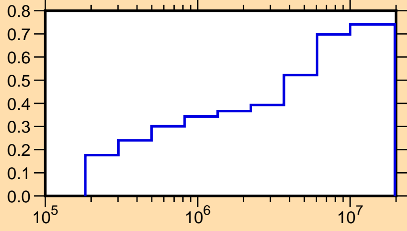
\mu vs. E for ^{36}\text{S}(\text{mt251})
