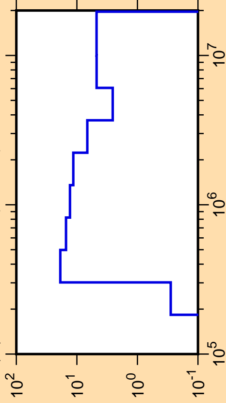
\Delta\mu/\mu vs. E for ^{36}\text{S}(\text{mt251})
