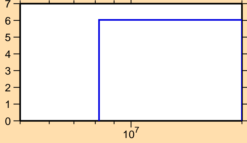
\Delta\sigma/\sigma vs. E for ^{36}\text{S}(n,el.)
