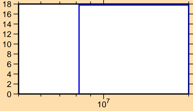
\Delta\sigma/\sigma vs. E for ^{36}\text{S}(n,ncont.)
