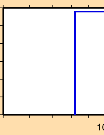
\sigma vs. E for ^{36}\text{S}(n,d)
