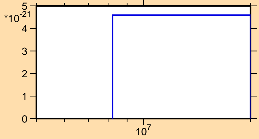
\sigma vs. E for ^{36}\text{S}(n,nd)
