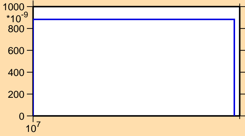
\sigma vs. E for ^{37}\text{S}(n,\text{nd})
