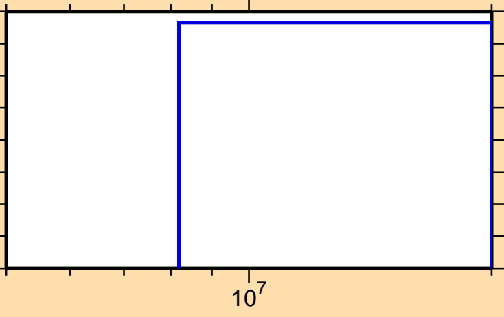
\sigma vs. E for ^{37}\text{S}(n,\text{nd})
