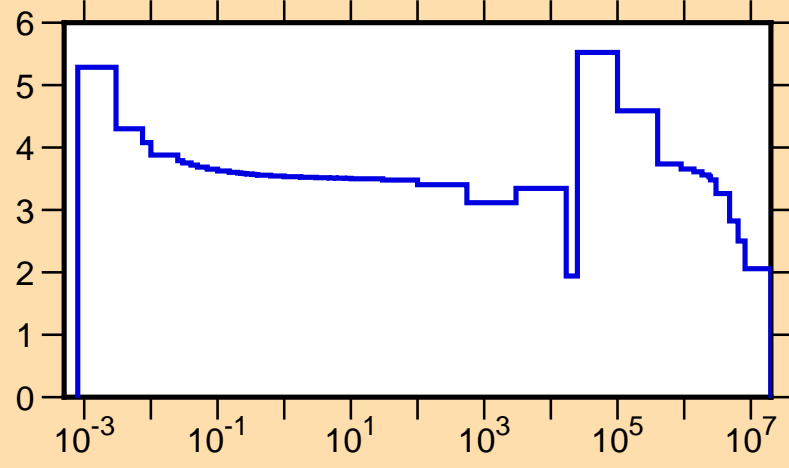
\sigma vs. E for ^{37}\text{S}(n,\text{tot.})
