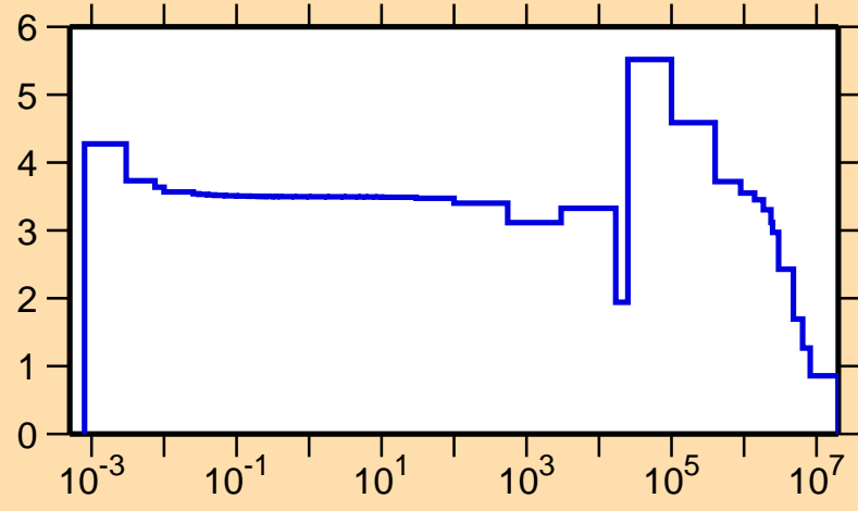
\sigma vs. E for ^{37}\text{S}(n,\text{el.})
