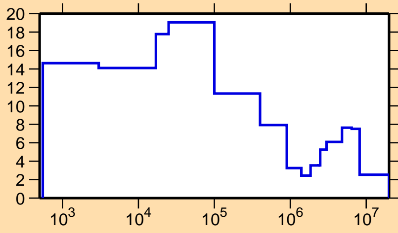
\Delta\sigma/\sigma vs. E for ^{37}\text{S}(n,\text{el.})
