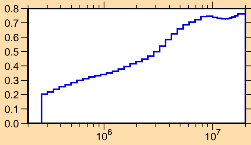
\mu vs. E for ^{38}\text{S}(\text{mt251})
