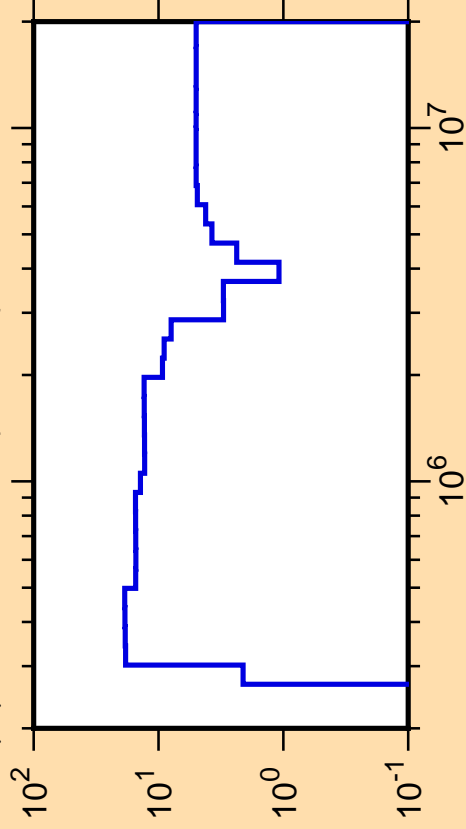
\Delta\mu/\mu vs. E for ^{38}\text{S}(\text{mt251})
