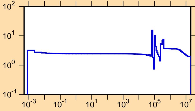
\sigma vs. E for ^{38}\text{S}(n,\text{tot.})
