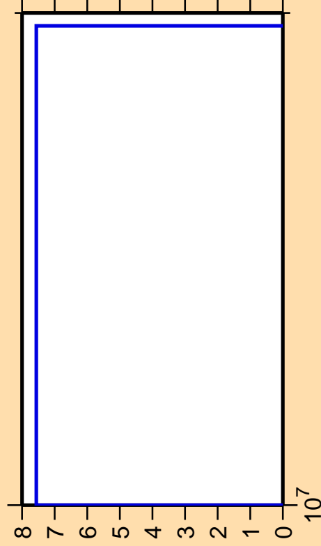
\Delta\sigma/\sigma vs. E for ^{38}\text{S}(n,3n)
