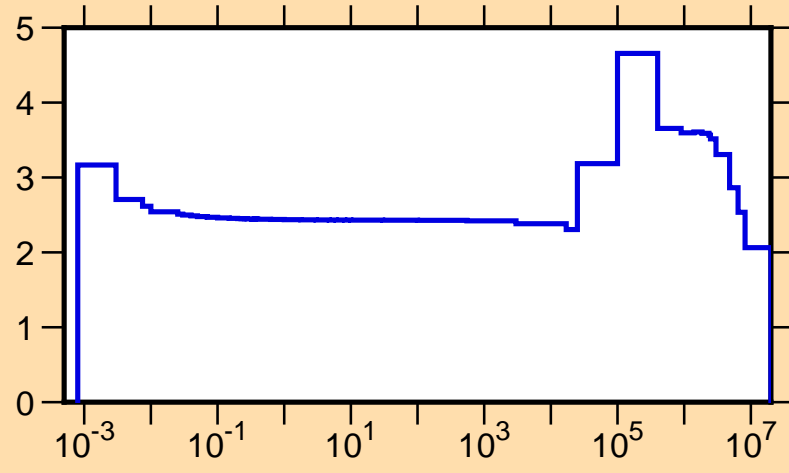
\sigma vs. E for ^{38}\text{S}(n,\text{tot.})
