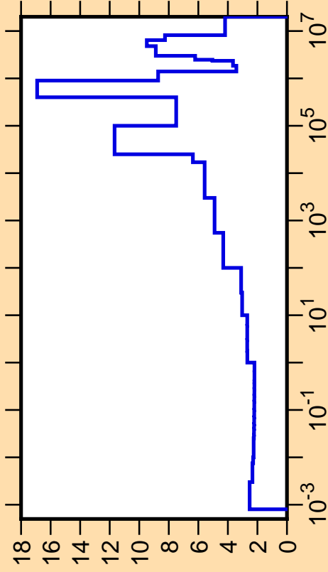
\Delta\sigma/\sigma vs. E for ^{38}\text{S}(n,\text{tot.})
