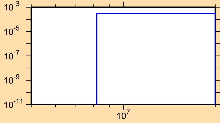
\sigma vs. E for ^{38}\text{S}(n,\alpha)
