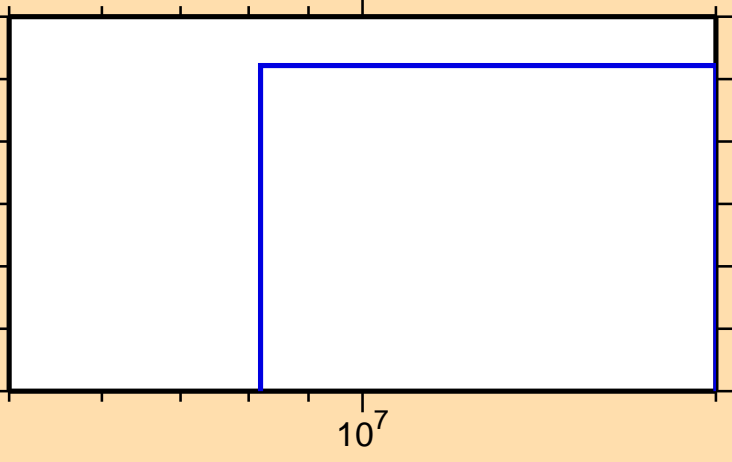
\sigma vs. E for ^{38}\text{S}(n,3n)
