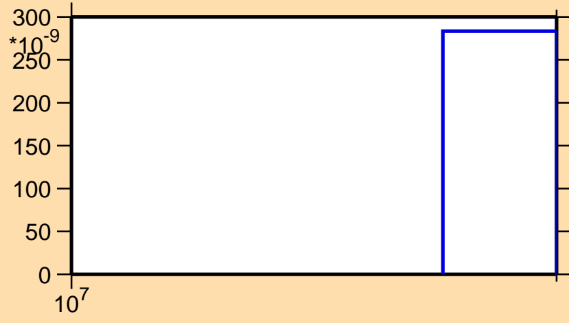
\sigma vs. E for ^{39}\text{S}(n,\text{nd})
