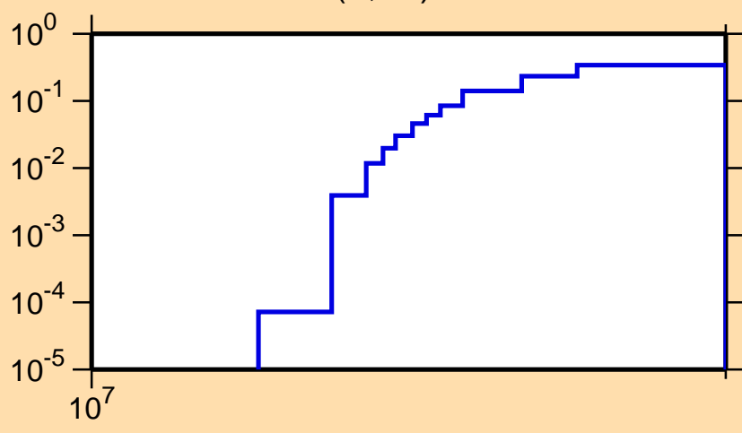
\sigma vs. E for ^{39}\text{S}(n,3n)
