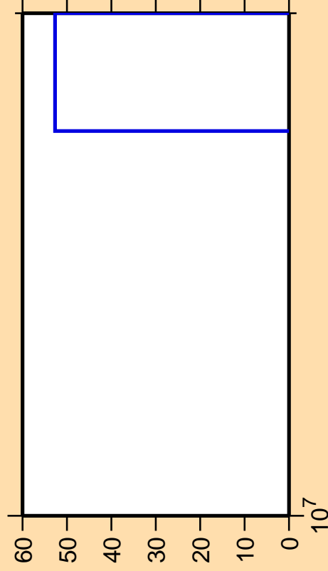
\Delta\sigma/\sigma vs. E for ^{39}\text{S}(n,\text{nd})
