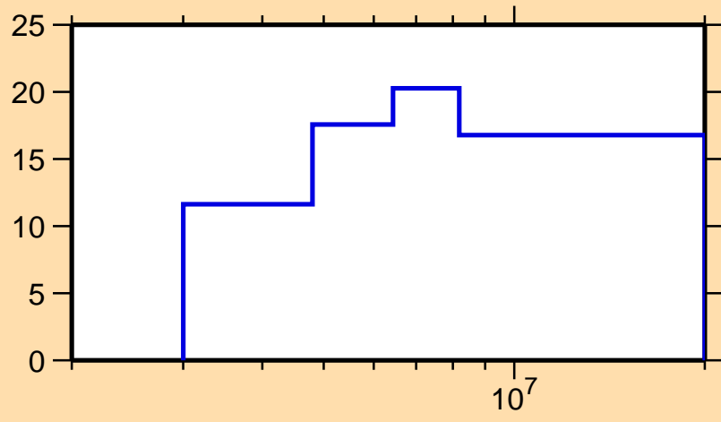
\Delta\sigma/\sigma vs. E for ^{39}\text{S}(n,n\text{onel.})
