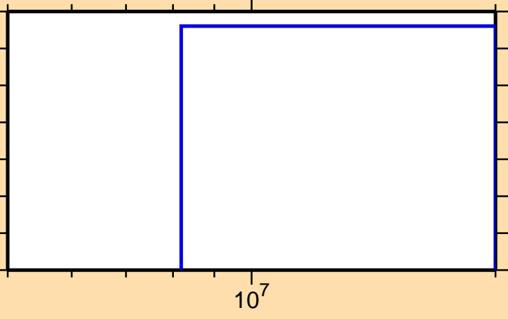
\sigma vs. E for ^{39}\text{S}(n,2n\alpha)
