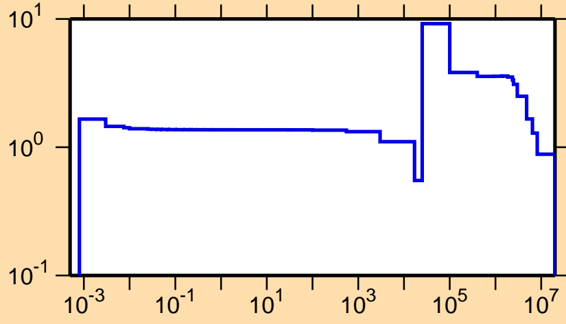
\sigma vs. E for ^{39}\text{S}(n,\text{el.})
