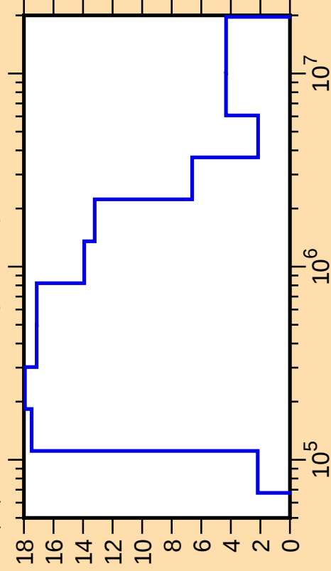
\Delta\mu/\mu vs. E for ^{41}\text{S}(\text{mt251})
