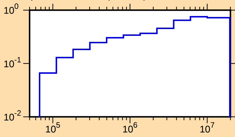
\mu vs. E for ^{41}\text{S}(\text{mt251})
