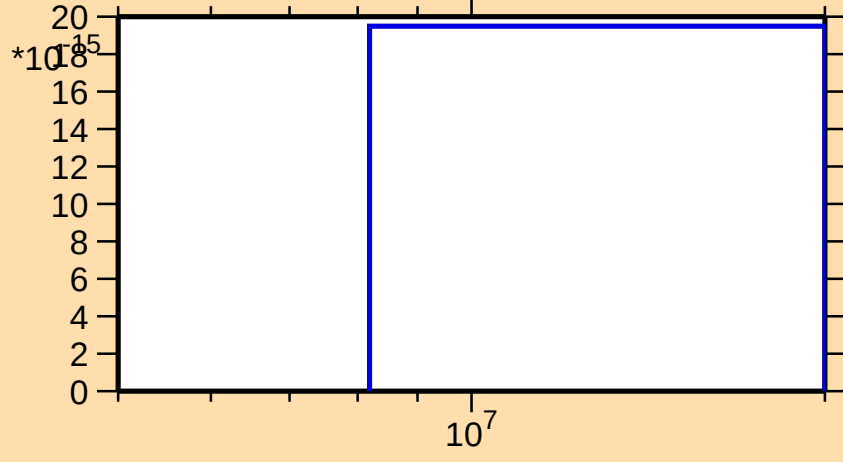
\sigma vs. E for ^{41}\text{S}(\text{n},\text{nt})
