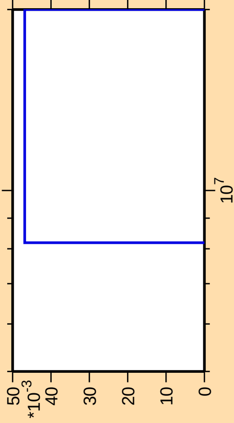
\Delta\sigma/\sigma vs. E for ^{41}\text{S}(\text{n},\text{nt})
