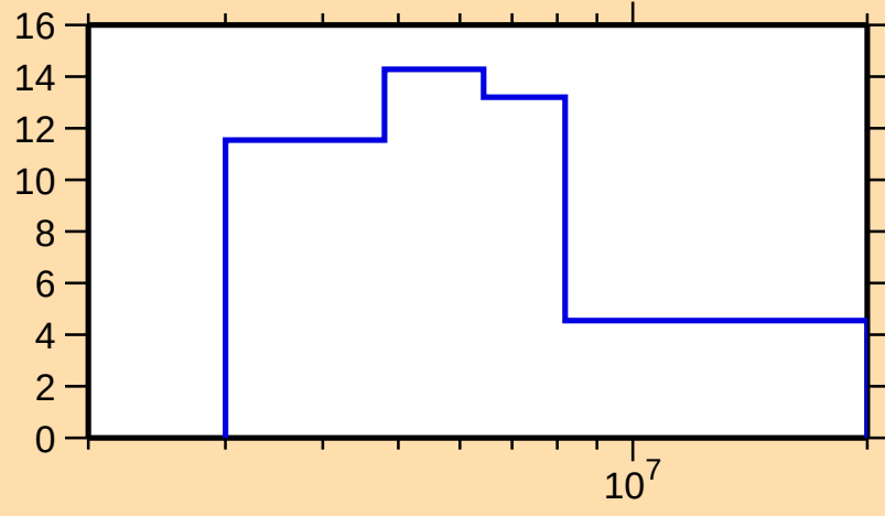
\Delta\sigma/\sigma vs. E for ^{41}\text{S}(\text{n},\text{el.})
