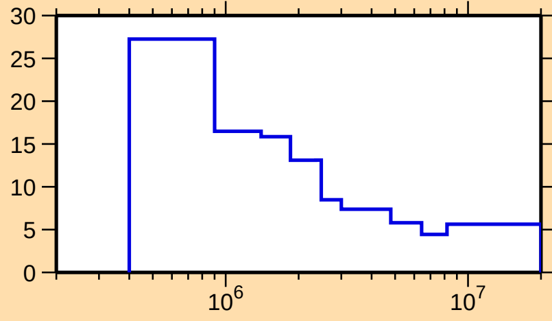
\Delta\sigma/\sigma vs. E for ^{41}\text{S}(\text{n,nonel.})
