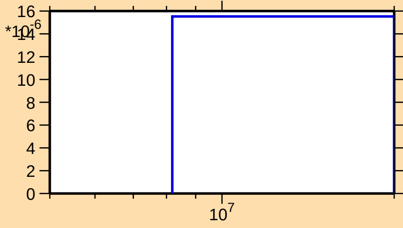
\sigma vs. E for ^{41}\text{S}(\text{n,p})
