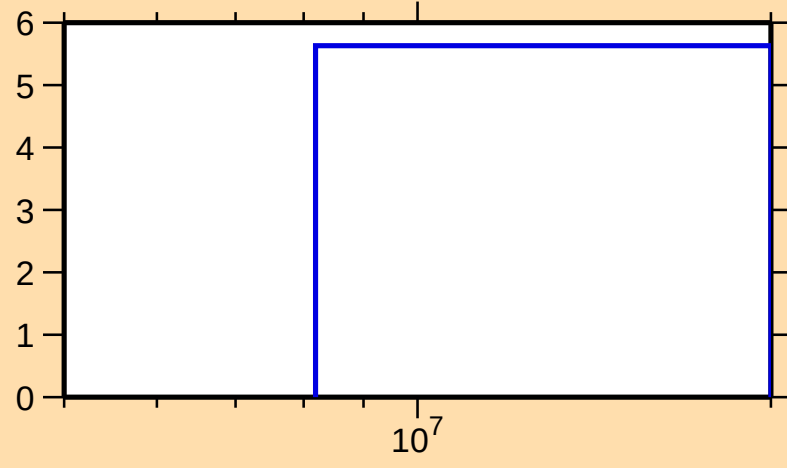
\Delta\sigma/\sigma vs. E for ^{41}\text{S}(\text{n,nonel.})
