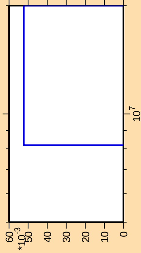
\Delta\sigma/\sigma vs. E for ^{41}\text{S}(\text{n},\text{nd})
