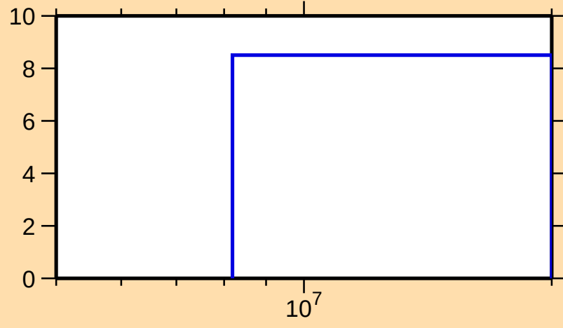
\Delta\sigma/\sigma vs. E for ^{41}\text{S}(\text{n},2\text{n})
