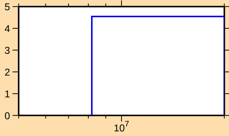
\Delta\sigma/\sigma vs. E for ^{41}\text{S}(\text{n,el.})
