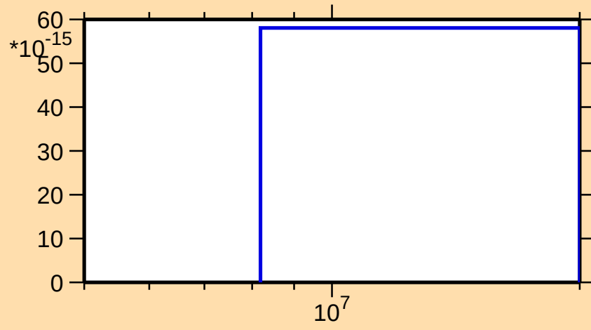
\sigma vs. E for ^{41}\text{S}(\text{n},\text{nd})
