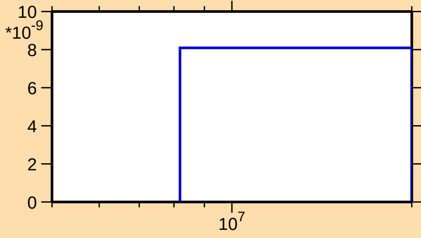
\sigma vs. E for ^{41}\text{S}(\text{n,d})
