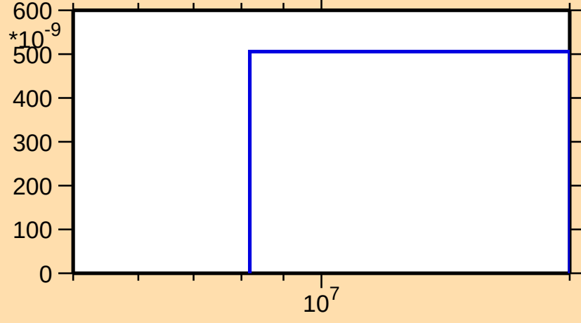
\sigma vs. E for ^{41}\text{S}(n,\alpha)
