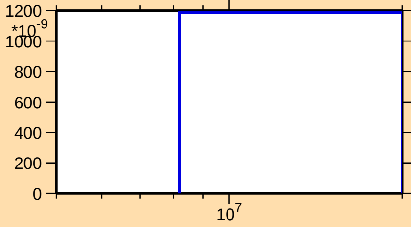
\sigma vs. E for ^{41}\text{S}(\text{n,t})
