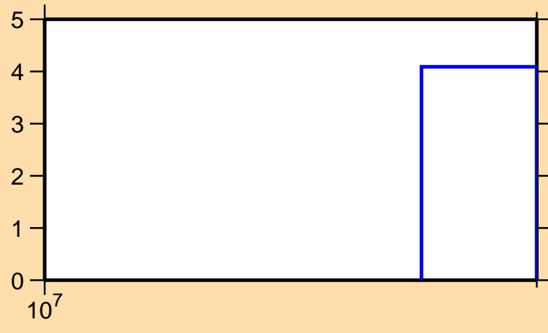
\Delta\sigma/\sigma vs. E for ^{42}\text{S}(n,\text{nonel.})
