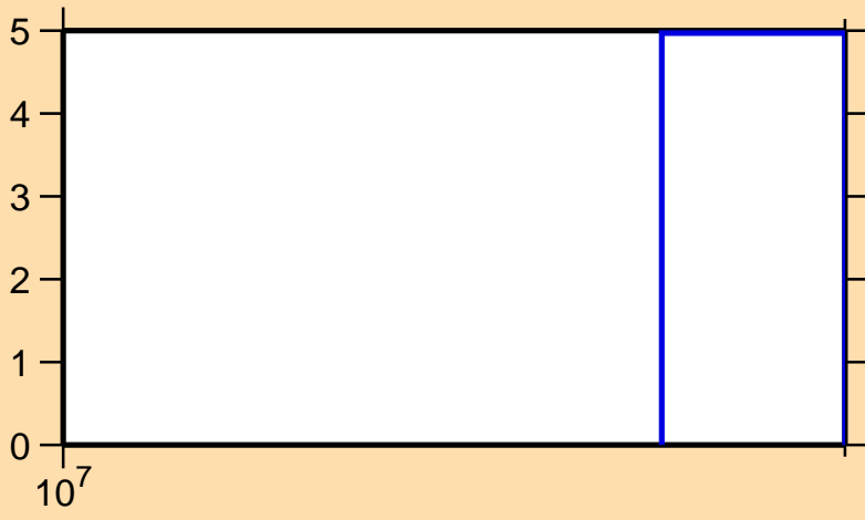
\Delta\sigma/\sigma vs. E for ^{42}\text{S}(n,\text{inel.})
