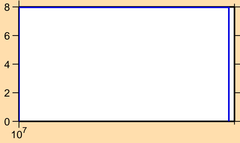
\Delta\sigma/\sigma vs. E for ^{42}\text{S}(n,2n)
