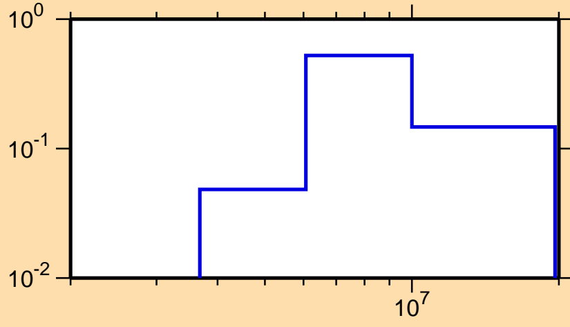
\sigma vs. E for ^{42}\text{S}(n,n\text{cont.})
