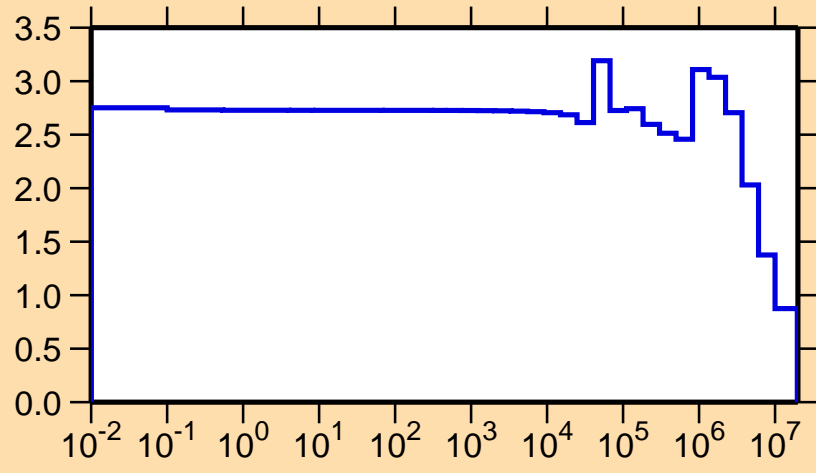
\sigma vs. E for ^{42}\text{S}(n,\text{el.})
