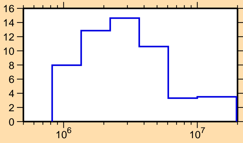
\Delta\sigma/\sigma vs. E for ^{42}\text{S}(n,\text{el.})
