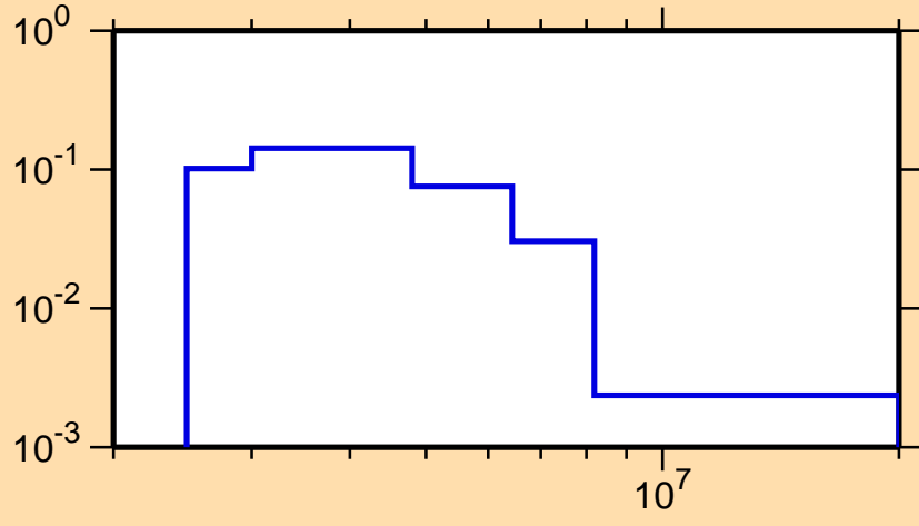
\sigma vs. E for ^{42}\text{S}(n,n_3)
