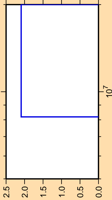
\Delta\sigma/\sigma vs. E for ^{42}\text{S}(n,p)
