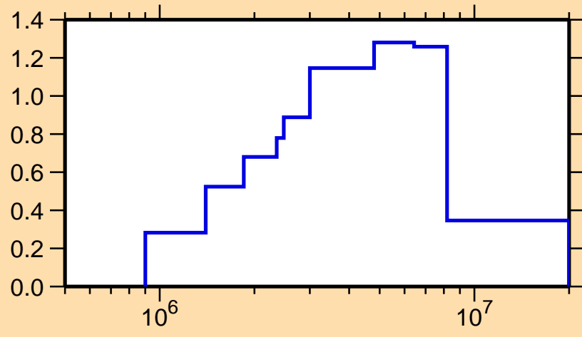
\sigma vs. E for ^{42}\text{S}(n,\text{inel.})
