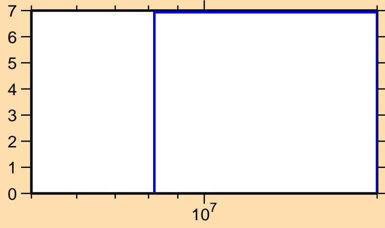
\Delta\sigma/\sigma vs. E for ^{42}\text{S}(n,\text{nonel.})
