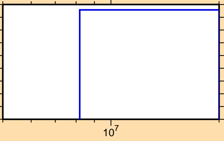
\sigma vs. E for ^{105}\text{Sb}(n,\text{pt})
