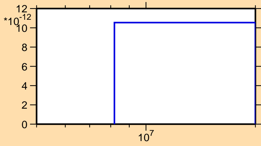
\sigma vs. E for ^{105}\text{Sb}(n,2n\alpha)
