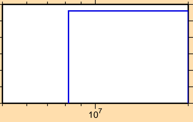
\sigma vs. E for ^{105}\text{Sb}(\text{mt } 34)
