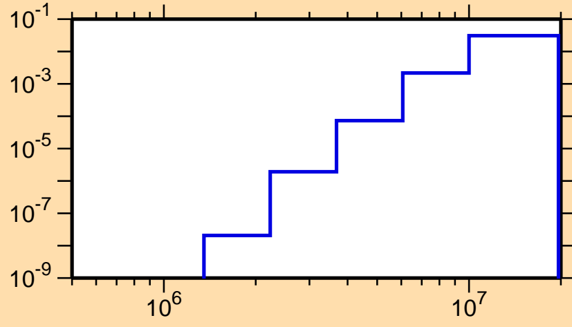
\sigma vs. E for ^{108}\text{Sb}(n,d)
