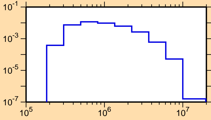
\sigma vs. E for ^{108}\text{Sb}(n,n_1)
