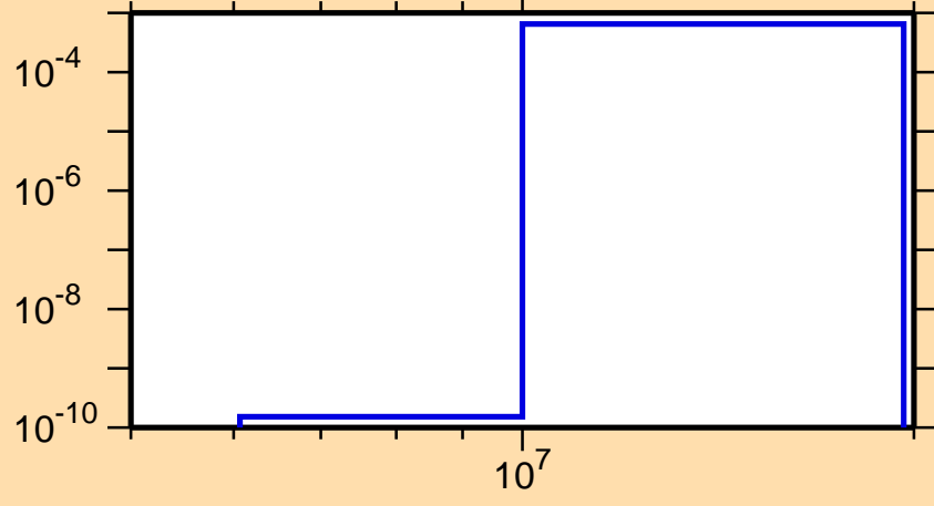
\sigma vs. E for ^{108}\text{Sb}(n,\text{pd})
